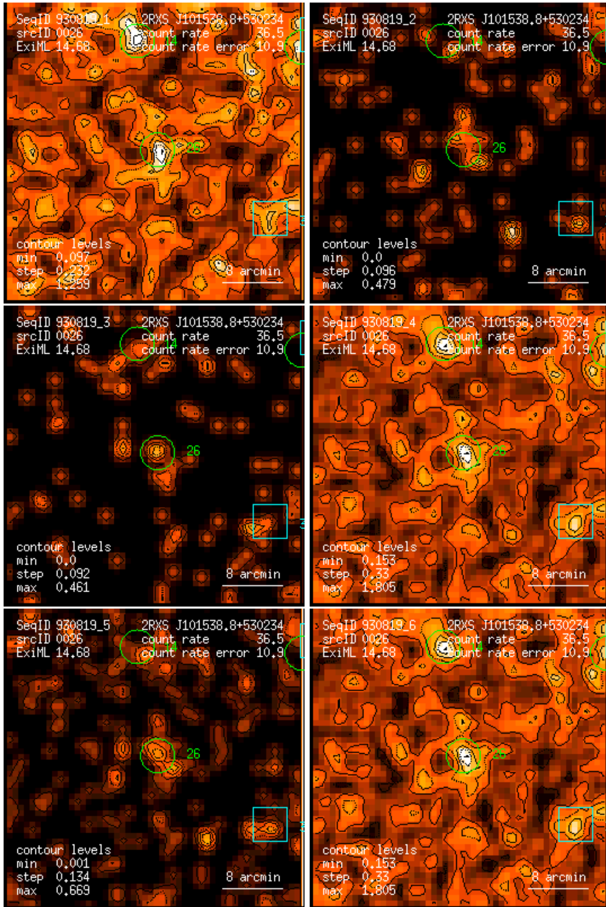
Figure 26: RASS 930819: detection 0026: band rate images, Gaussian filter: (1) PSPC channels 11 – 41, (2) 52 – 90, (3) 91 – 201, (4) 11 – 235, (5) 52 – 201, (6) 11 – 201. Broad band rates in counts/ks. Band rate contour levels in counts/ks/arcmin 2 .
