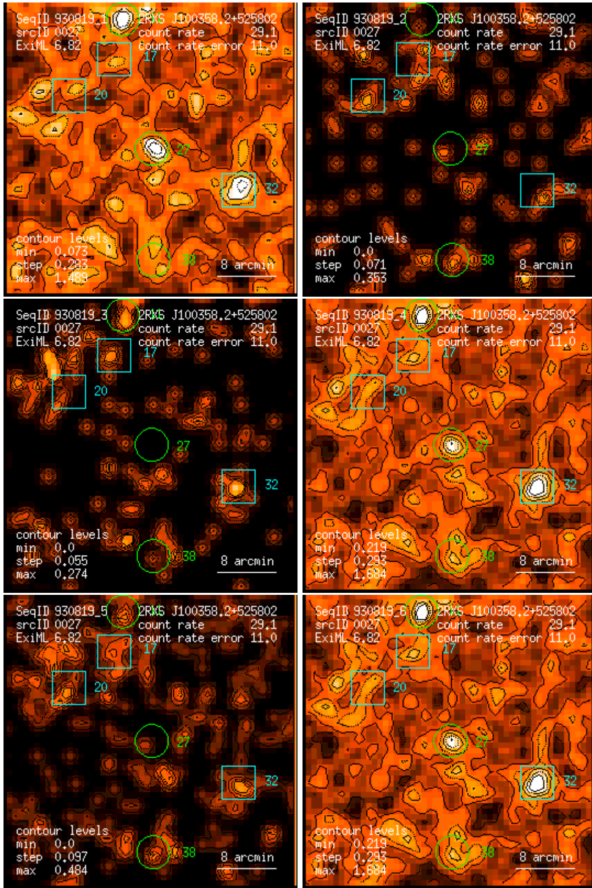
Figure 27: RASS 930819: detection 0027: band rate images, Gaussian filter: (1) PSPC channels 11 – 41, (2) 52 – 90, (3) 91 – 201, (4) 11 – 235, (5) 52 – 201, (6) 11 – 201. Broad band rates in counts/ks. Band rate contour levels in counts/ks/arcmin 2 .
