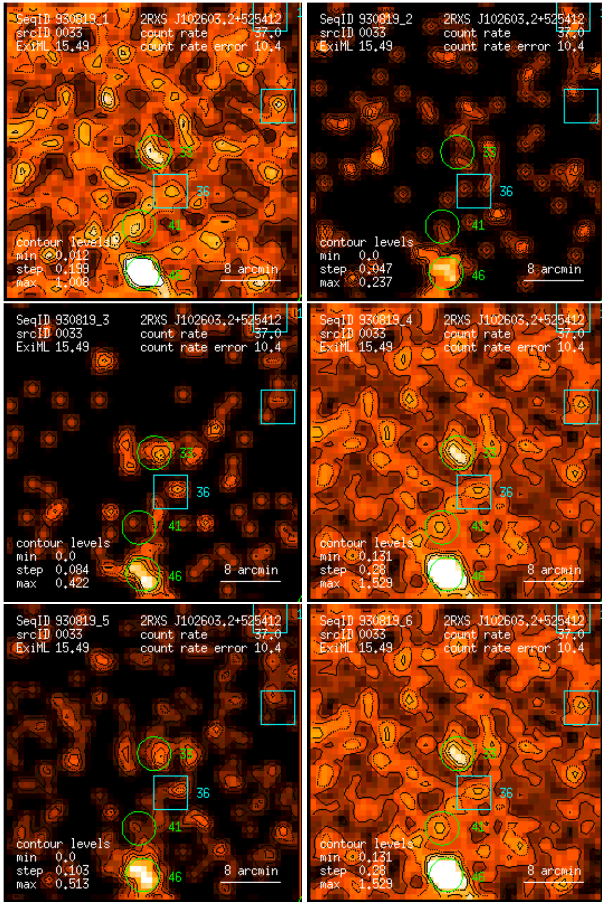
Figure 33: RASS 930819: detection 0033: band rate images, Gaussian filter: (1) PSPC channels 11 – 41, (2) 52 – 90, (3) 91 – 201, (4) 11 – 235, (5) 52 – 201, (6) 11 – 201. Broad band rates in counts/ks. Band rate contour levels in counts/ks/arcmin 2 .
