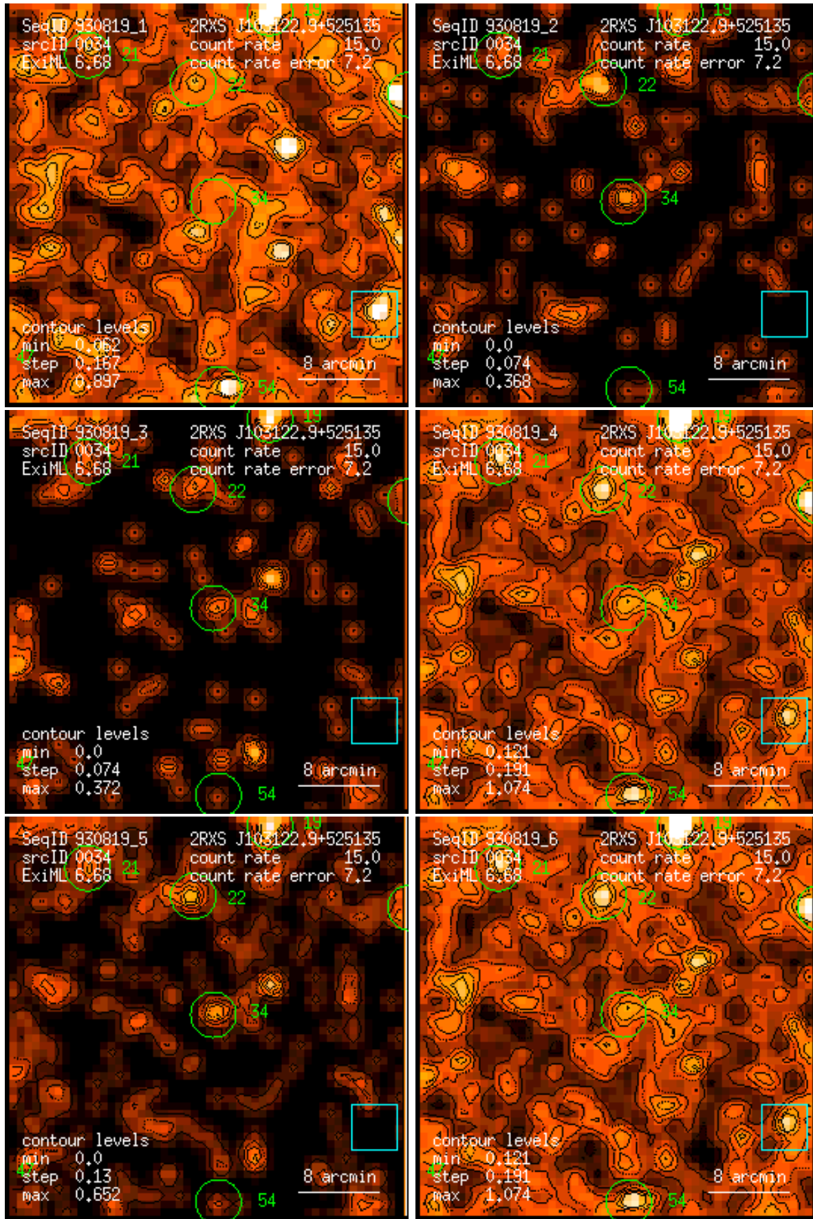
Figure 34: RASS 930819: detection 0034: band rate images, Gaussian filter: (1) PSPC channels 11 – 41, (2) 52 – 90, (3) 91 – 201, (4) 11 – 235, (5) 52 – 201, (6) 11 – 201. Broad band rates in counts/ks. Band rate contour levels in counts/ks/arcmin 2 .
