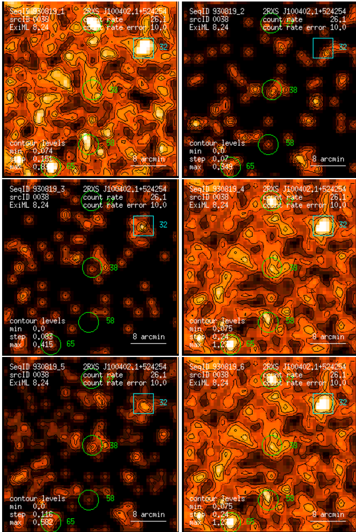
Figure 38: RASS 930819: detection 0038: band rate images, Gaussian filter: (1) PSPC channels 11 – 41, (2) 52 – 90, (3) 91 – 201, (4) 11 – 235, (5) 52 – 201, (6) 11 – 201. Broad band rates in counts/ks. Band rate contour levels in counts/ks/arcmin 2 .
