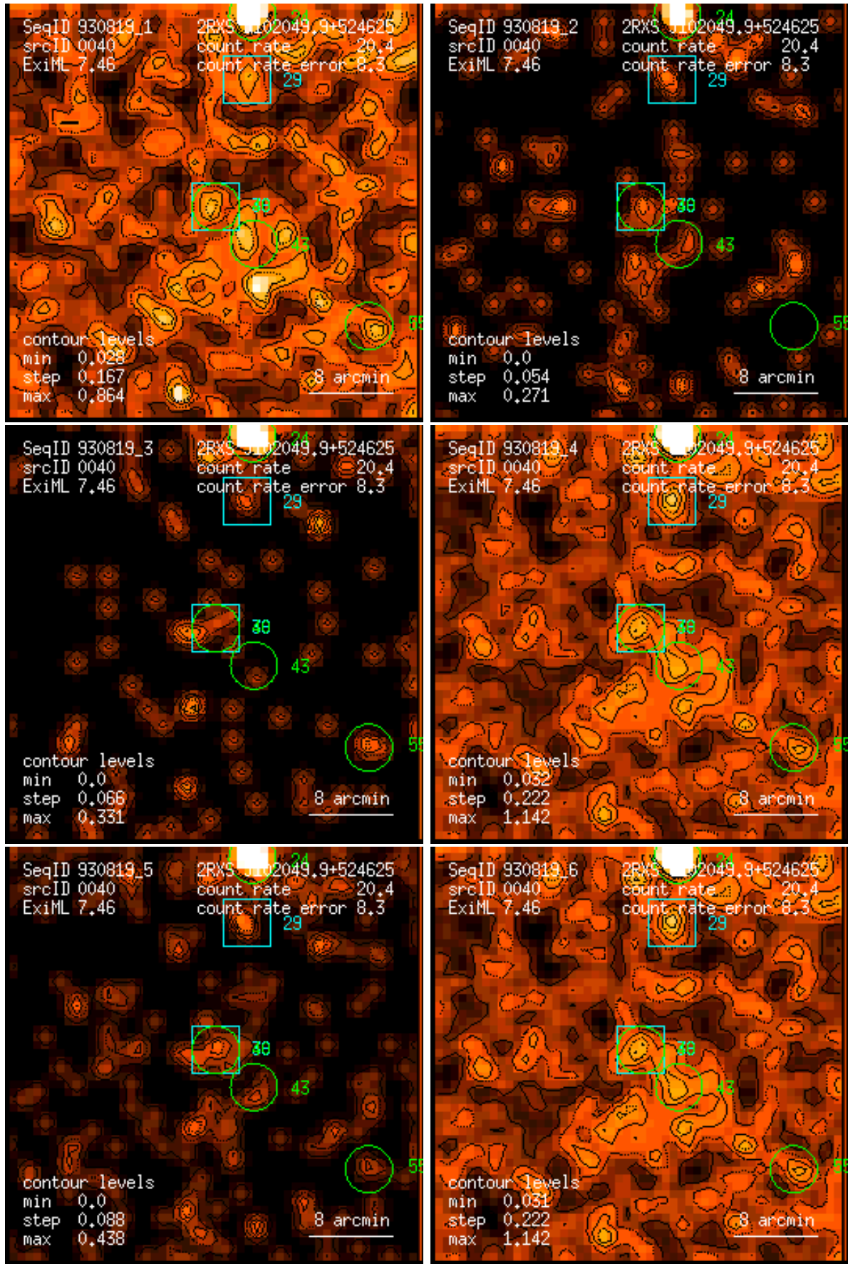
Figure 40: RASS 930819: detection 0040: band rate images, Gaussian filter: (1) PSPC channels 11 – 41, (2) 52 – 90, (3) 91 – 201, (4) 11 – 235, (5) 52 – 201, (6) 11 – 201. Broad band rates in counts/ks. Band rate contour levels in counts/ks/arcmin 2 .
