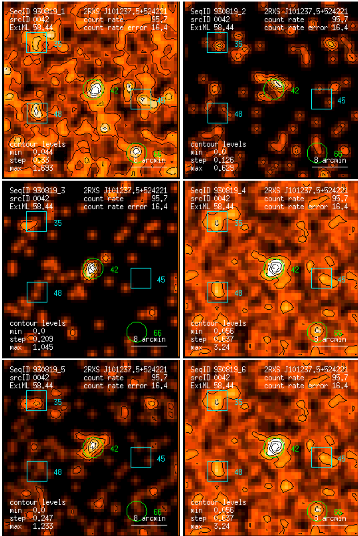
Figure 42: RASS 930819: detection 0042: band rate images, Gaussian filter: (1) PSPC channels 11 – 41, (2) 52 – 90, (3) 91 – 201, (4) 11 – 235, (5) 52 – 201, (6) 11 – 201. Broad band rates in counts/ks. Band rate contour levels in counts/ks/arcmin 2 .
