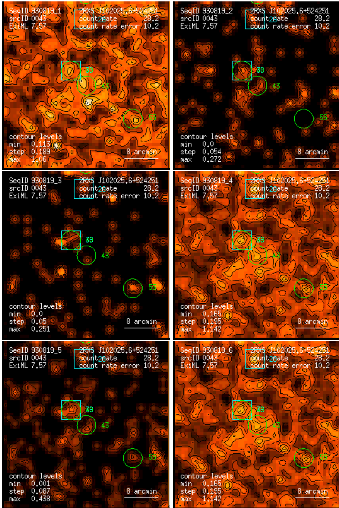
Figure 43: RASS 930819: detection 0043: band rate images, Gaussian filter: (1) PSPC channels 11 – 41, (2) 52 – 90, (3) 91 – 201, (4) 11 – 235, (5) 52 – 201, (6) 11 – 201. Broad band rates in counts/ks. Band rate contour levels in counts/ks/arcmin 2 .
