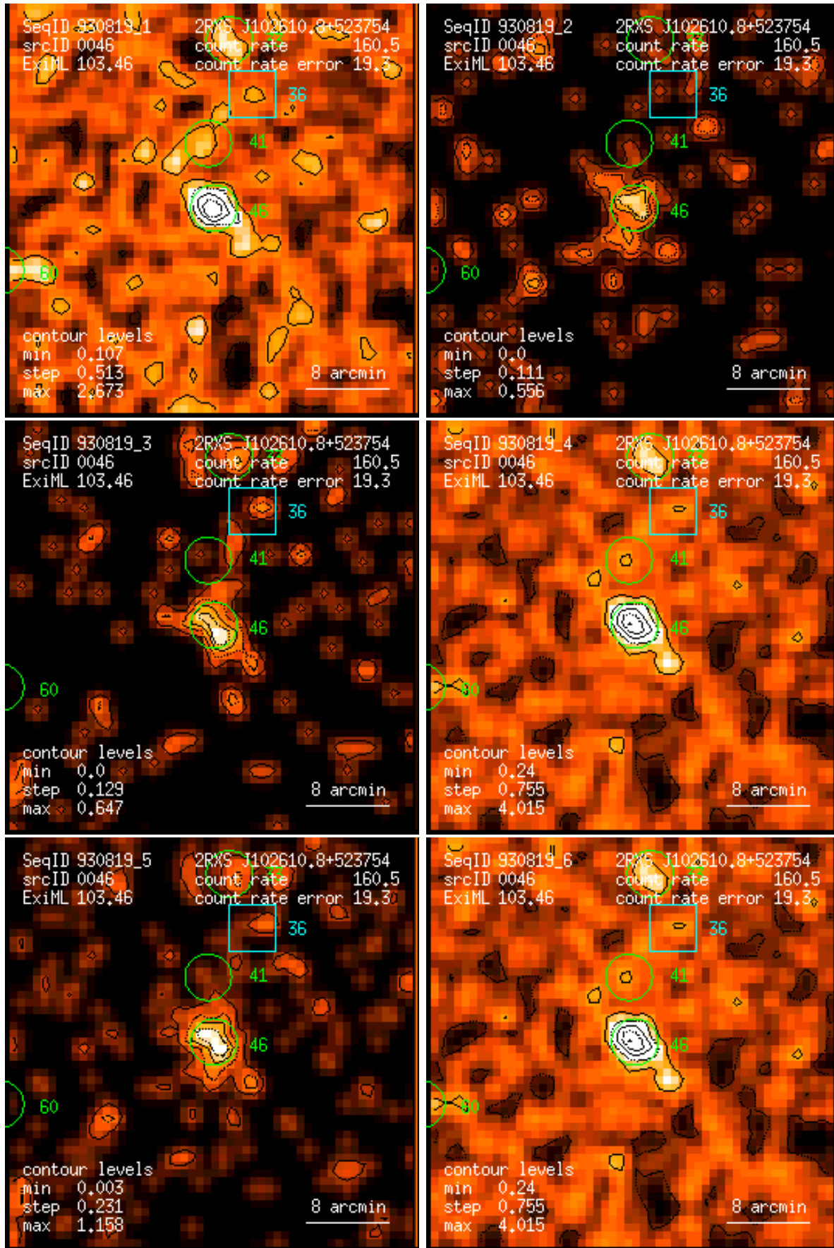
Figure 46: RASS 930819: detection 0046: band rate images, Gaussian filter: (1) PSPC channels 11 – 41, (2) 52 – 90, (3) 91 – 201, (4) 11 – 235, (5) 52 – 201, (6) 11 – 201. Broad band rates in counts/ks. Band rate contour levels in counts/ks/arcmin 2 .
