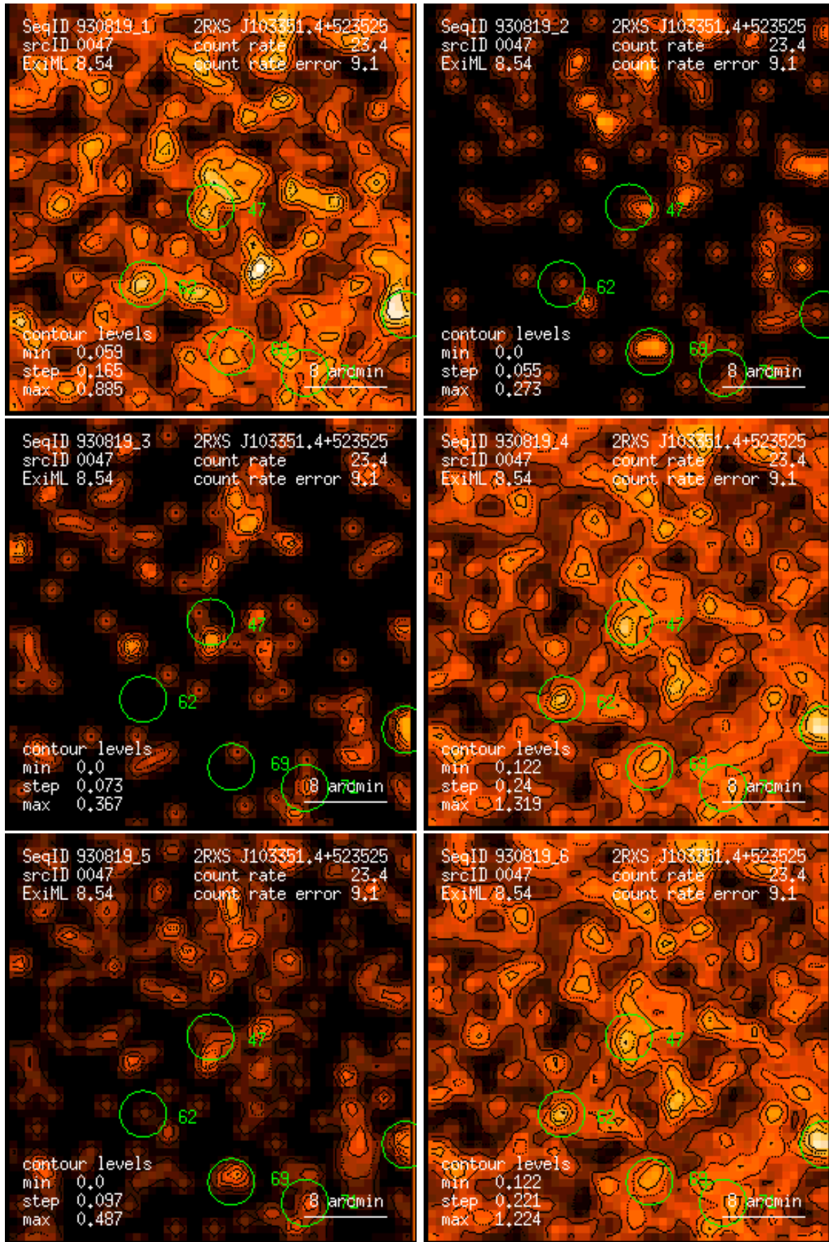
Figure 47: RASS 930819: detection 0047: band rate images, Gaussian filter: (1) PSPC channels 11 – 41, (2) 52 – 90, (3) 91 – 201, (4) 11 – 235, (5) 52 – 201, (6) 11 – 201. Broad band rates in counts/ks. Band rate contour levels in counts/ks/arcmin 2 .
