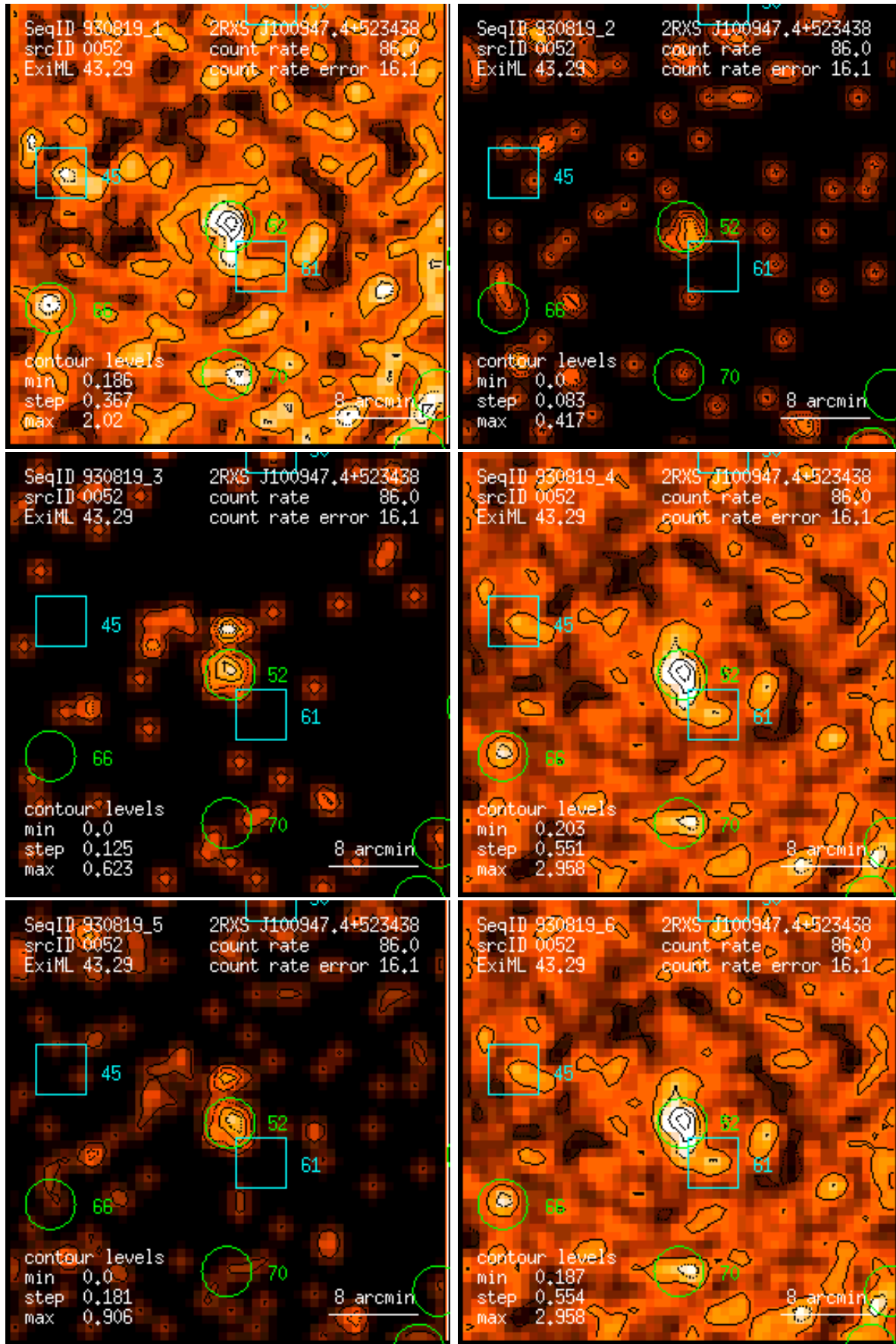
Figure 52: RASS 930819: detection 0052: band rate images, Gaussian filter: (1) PSPC channels 11 – 41, (2) 52 – 90, (3) 91 – 201, (4) 11 – 235, (5) 52 – 201, (6) 11 – 201. Broad band rates in counts/ks. Band rate contour levels in counts/ks/arcmin 2 .
