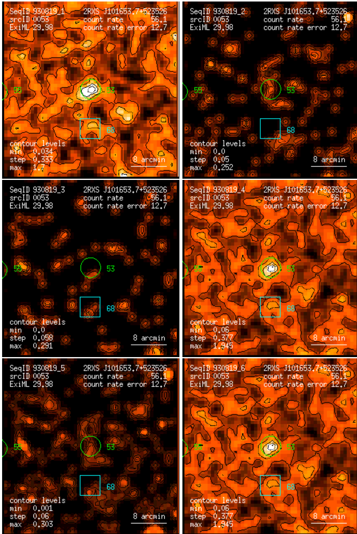
Figure 53: RASS 930819: detection 0053: band rate images, Gaussian filter: (1) PSPC channels 11 – 41, (2) 52 – 90, (3) 91 – 201, (4) 11 – 235, (5) 52 – 201, (6) 11 – 201. Broad band rates in counts/ks. Band rate contour levels in counts/ks/arcmin 2 .
