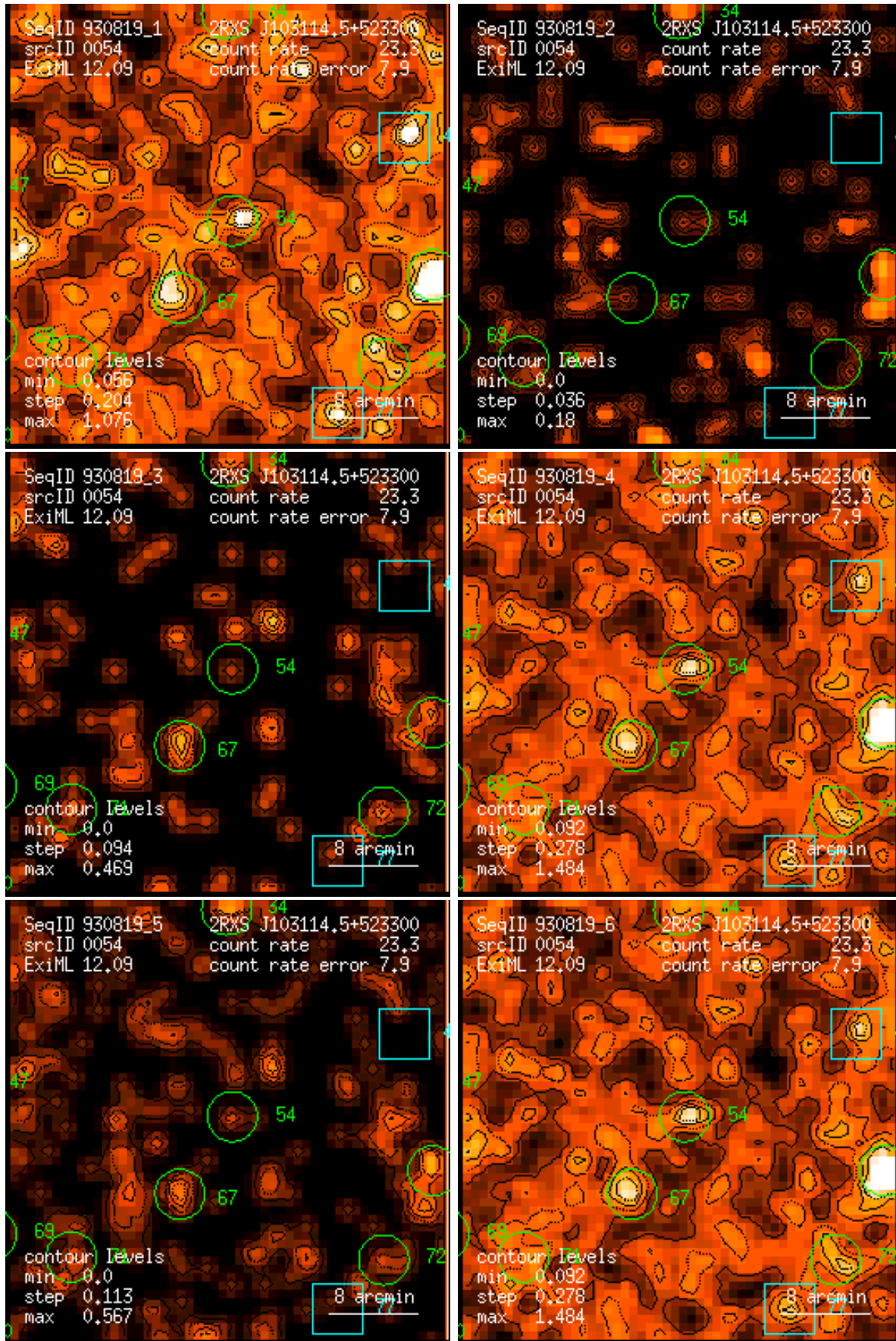
Figure 54: RASS 930819: detection 0054: band rate images, Gaussian filter: (1) PSPC channels 11 – 41, (2) 52 – 90, (3) 91 – 201, (4) 11 – 235, (5) 52 – 201, (6) 11 – 201. Broad band rates in counts/ks. Band rate contour levels in counts/ks/arcmin 2 .
