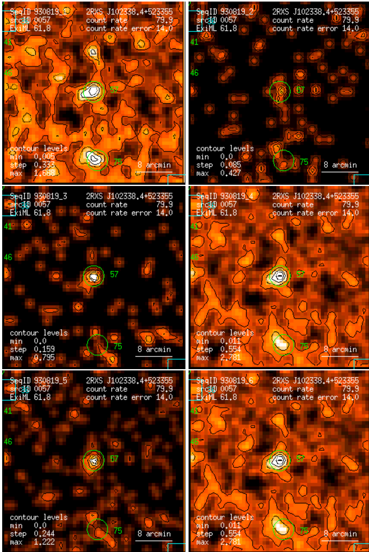
Figure 57: RASS 930819: detection 0057: band rate images, Gaussian filter: (1) PSPC channels 11 – 41, (2) 52 – 90, (3) 91 – 201, (4) 11 – 235, (5) 52 – 201, (6) 11 – 201. Broad band rates in counts/ks. Band rate contour levels in counts/ks/arcmin 2 .
