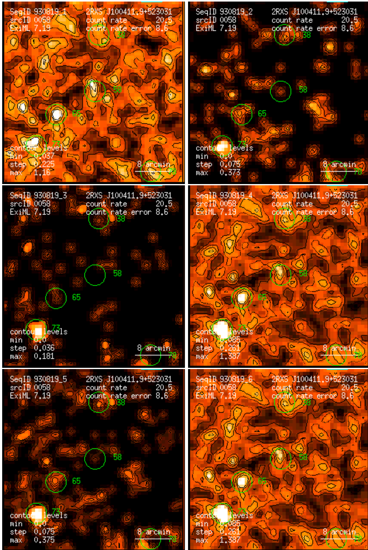
Figure 58: RASS 930819: detection 0058: band rate images, Gaussian filter: (1) PSPC channels 11 – 41, (2) 52 – 90, (3) 91 – 201, (4) 11 – 235, (5) 52 – 201, (6) 11 – 201. Broad band rates in counts/ks. Band rate contour levels in counts/ks/arcmin 2 .
