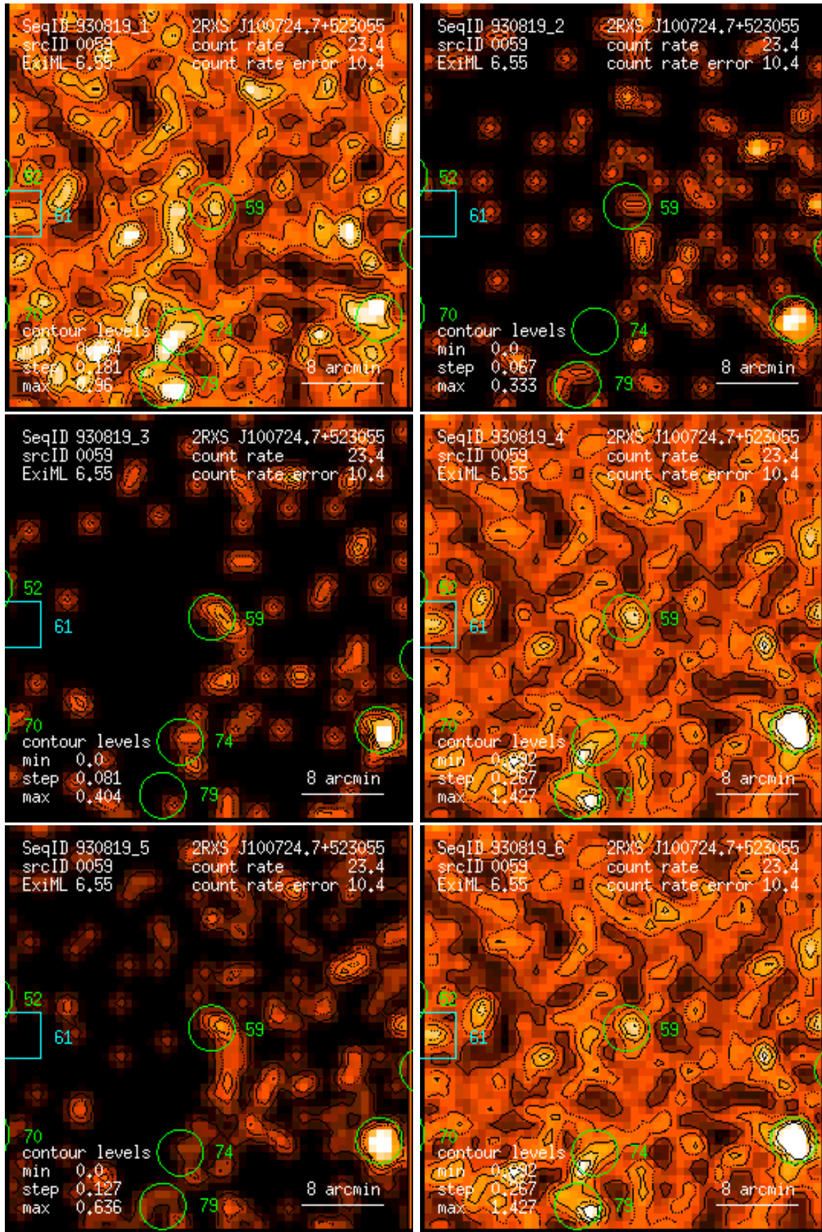
Figure 59: RASS 930819: detection 0059: band rate images, Gaussian filter: (1) PSPC channels 11 – 41, (2) 52 – 90, (3) 91 – 201, (4) 11 – 235, (5) 52 – 201, (6) 11 – 201. Broad band rates in counts/ks. Band rate contour levels in counts/ks/arcmin 2 .
