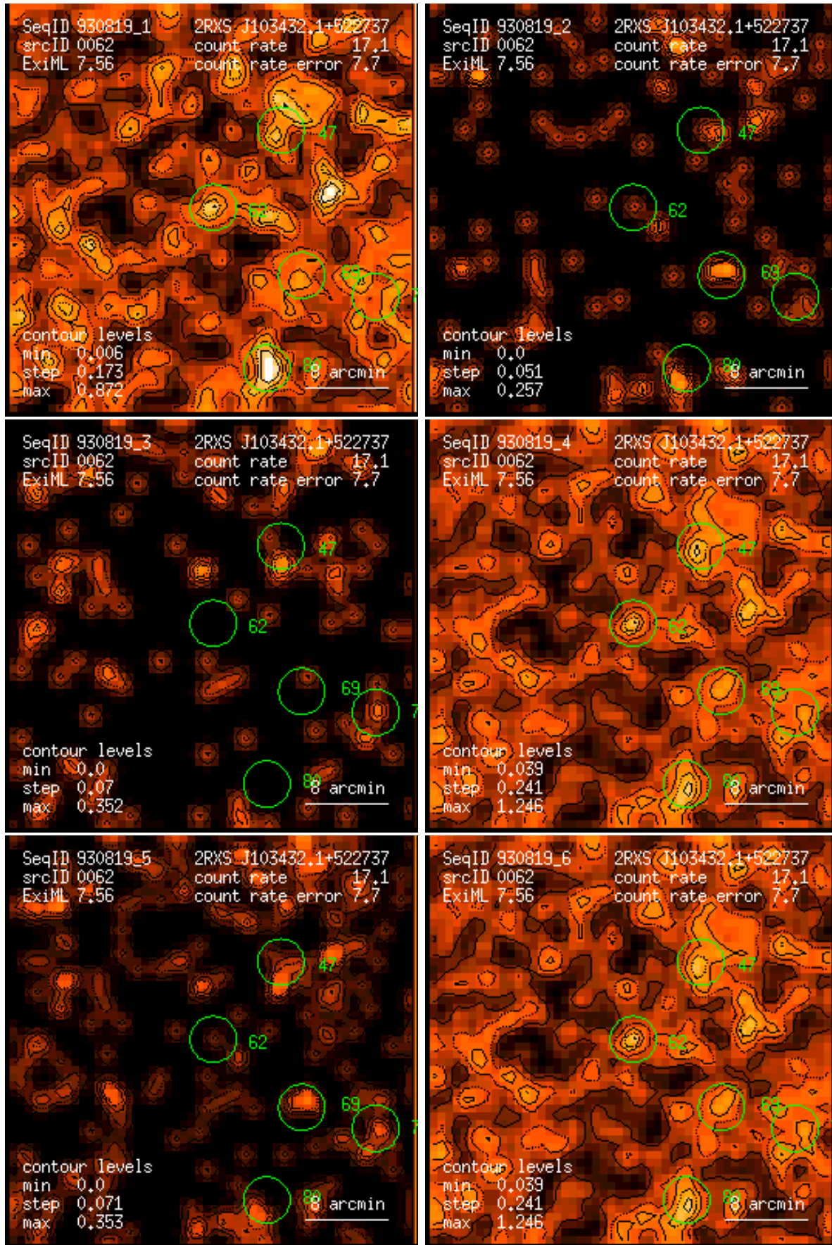
Figure 62: RASS 930819: detection 0062: band rate images, Gaussian filter: (1) PSPC channels 11 – 41, (2) 52 – 90, (3) 91 – 201, (4) 11 – 235, (5) 52 – 201, (6) 11 – 201. Broad band rates in counts/ks. Band rate contour levels in counts/ks/arcmin 2 .
