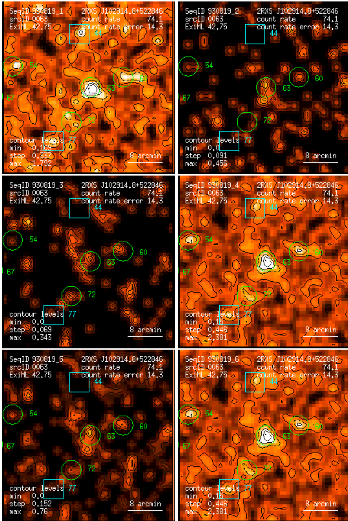
Figure 63: RASS 930819: detection 0063: band rate images, Gaussian filter: (1) PSPC channels 11 – 41, (2) 52 – 90, (3) 91 – 201, (4) 11 – 235, (5) 52 – 201, (6) 11 – 201. Broad band rates in counts/ks. Band rate contour levels in counts/ks/arcmin 2 .
