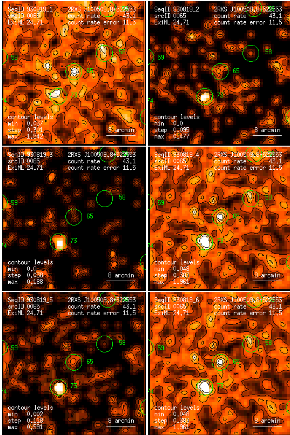
Figure 65: RASS 930819: detection 0065: band rate images, Gaussian filter: (1) PSPC channels 11 – 41, (2) 52 – 90, (3) 91 – 201, (4) 11 – 235, (5) 52 – 201, (6) 11 – 201. Broad band rates in counts/ks. Band rate contour levels in counts/ks/arcmin 2 .
