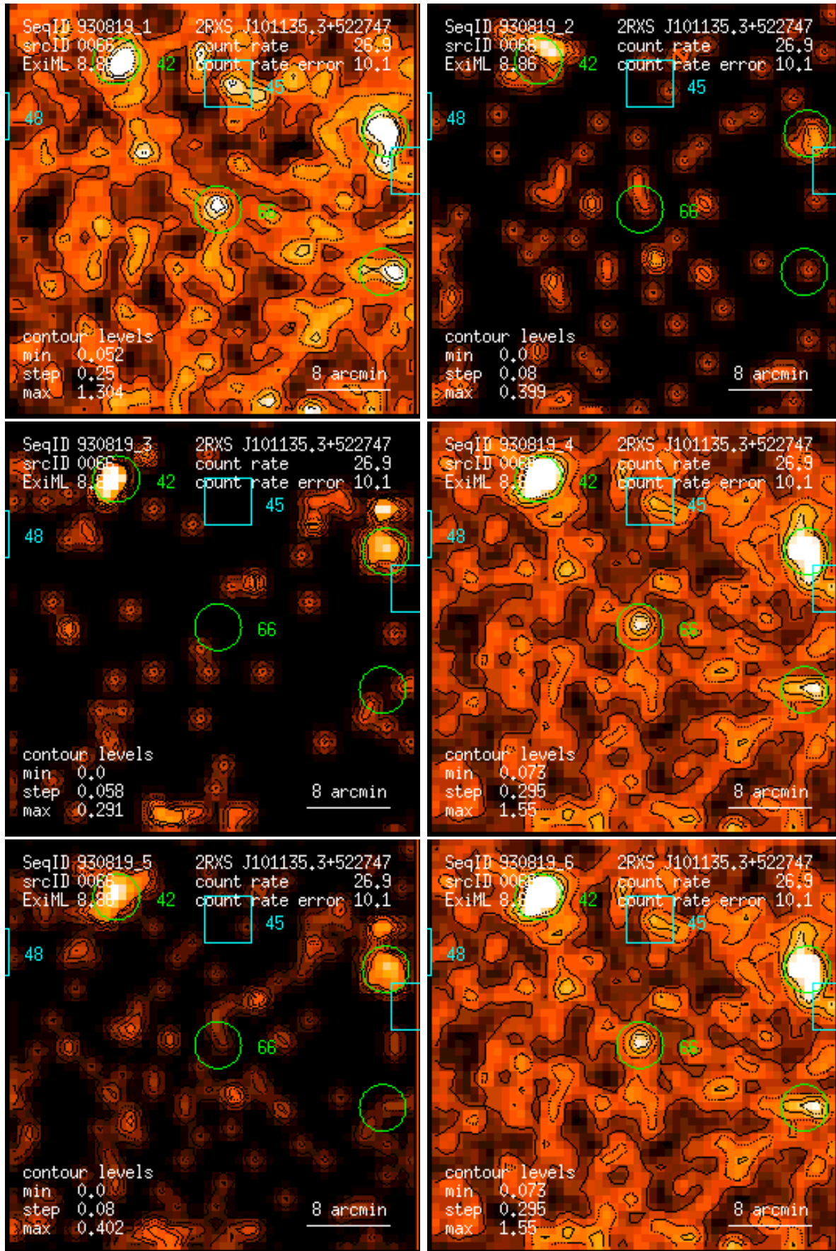
Figure 66: RASS 930819: detection 0066: band rate images, Gaussian filter: (1) PSPC channels 11 – 41, (2) 52 – 90, (3) 91 – 201, (4) 11 – 235, (5) 52 – 201, (6) 11 – 201. Broad band rates in counts/ks. Band rate contour levels in counts/ks/arcmin 2 .
