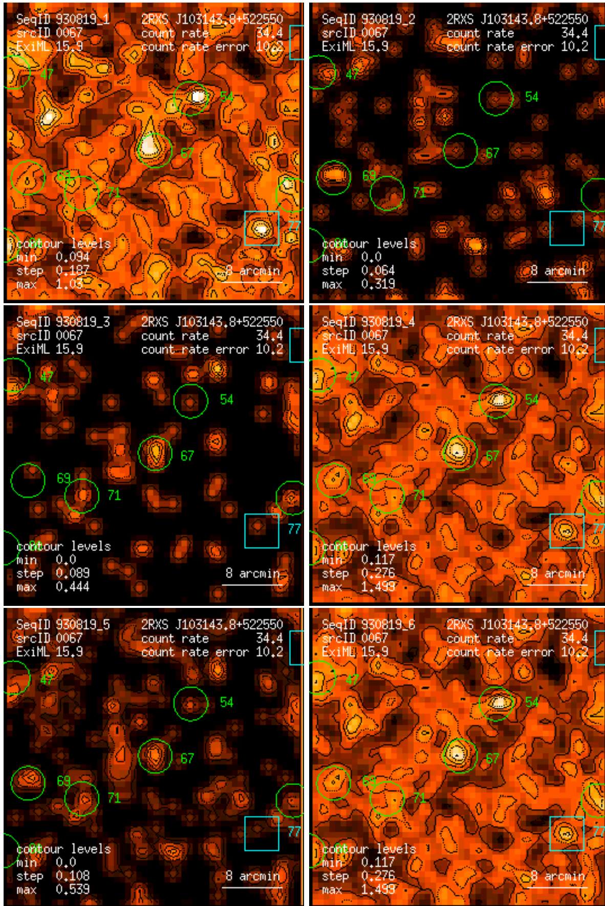
Figure 67: RASS 930819: detection 0067: band rate images, Gaussian filter: (1) PSPC channels 11 – 41, (2) 52 – 90, (3) 91 – 201, (4) 11 – 235, (5) 52 – 201, (6) 11 – 201. Broad band rates in counts/ks. Band rate contour levels in counts/ks/arcmin 2 .
