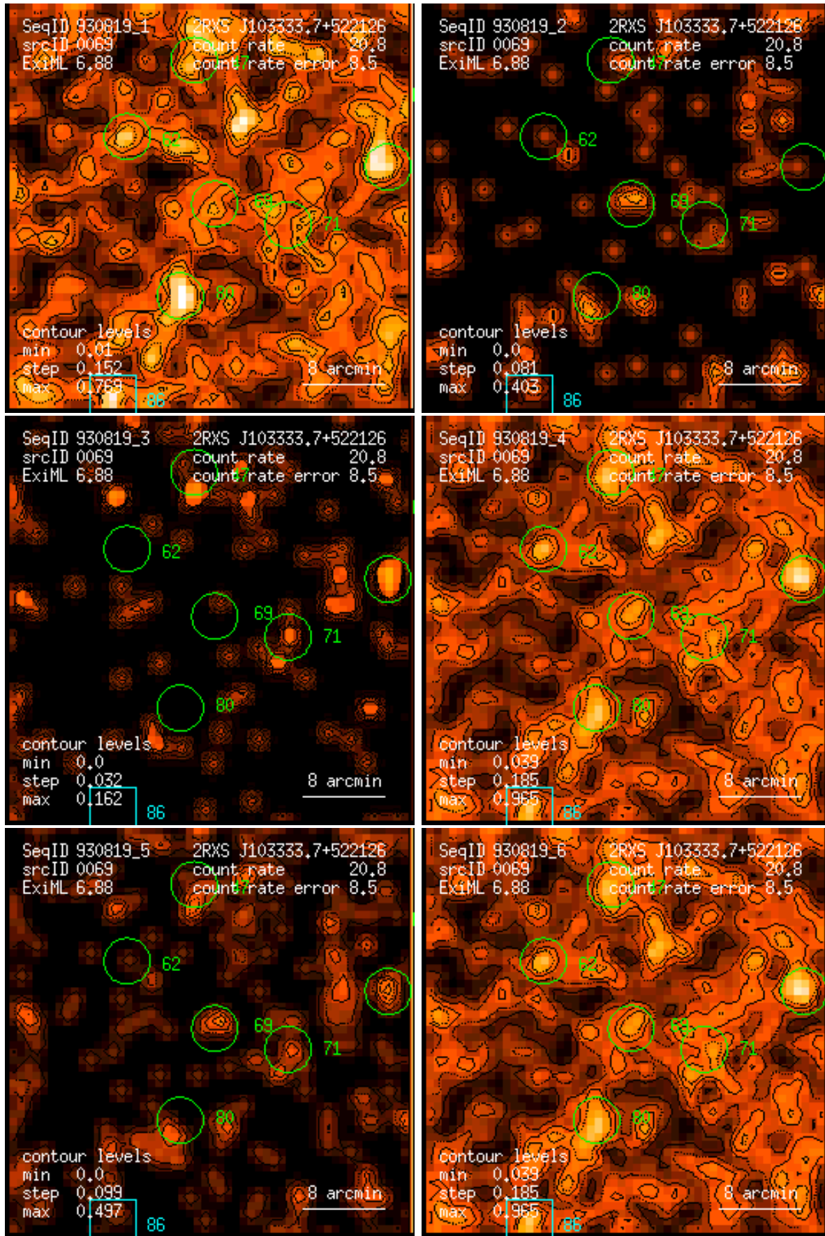
Figure 69: RASS 930819: detection 0069: band rate images, Gaussian filter: (1) PSPC channels 11 – 41, (2) 52 – 90, (3) 91 – 201, (4) 11 – 235, (5) 52 – 201, (6) 11 – 201. Broad band rates in counts/ks. Band rate contour levels in counts/ks/arcmin 2 .
