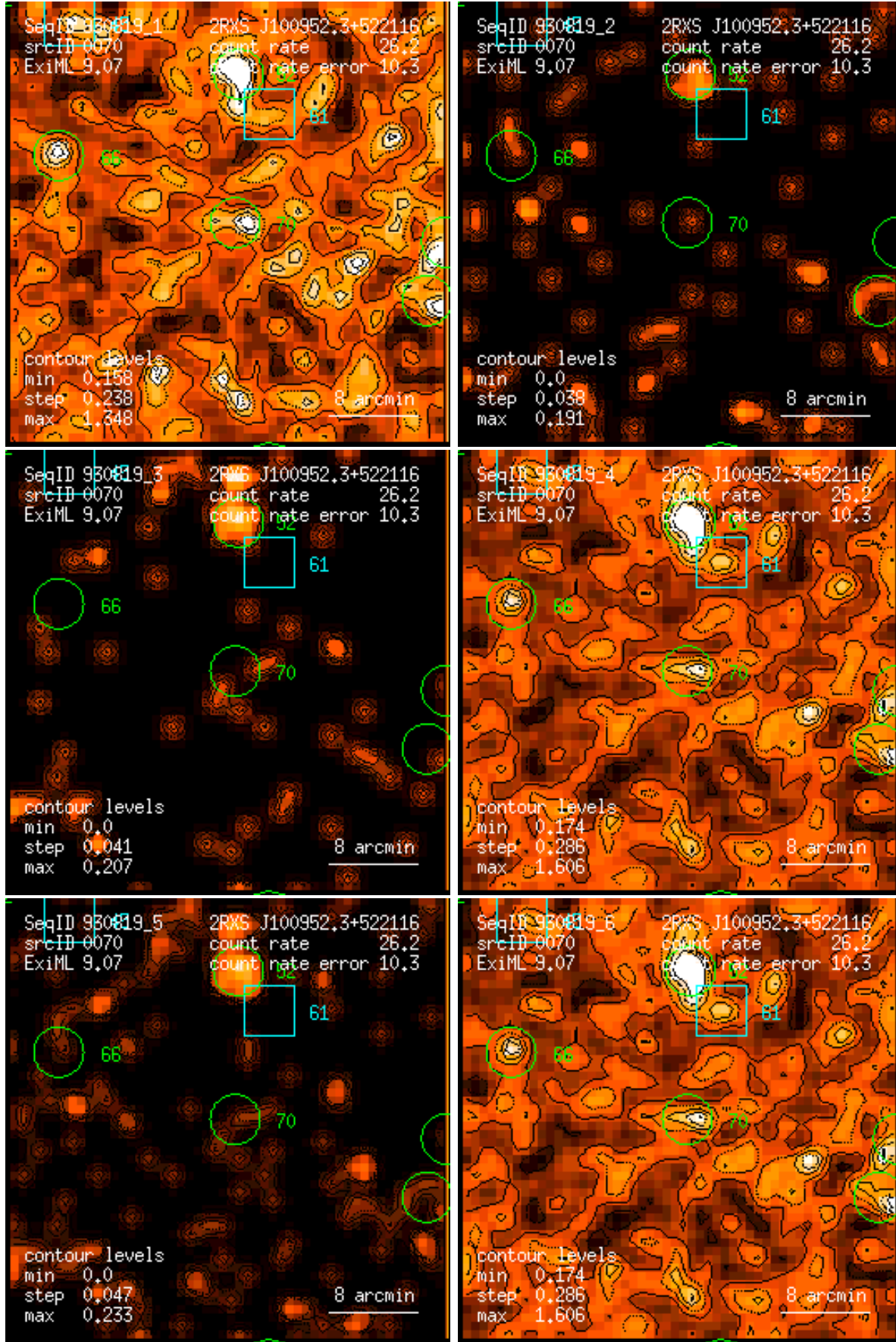
Figure 70: RASS 930819: detection 0070: band rate images, Gaussian filter: (1) PSPC channels 11 – 41, (2) 52 – 90, (3) 91 – 201, (4) 11 – 235, (5) 52 – 201, (6) 11 – 201. Broad band rates in counts/ks. Band rate contour levels in counts/ks/arcmin 2 .
