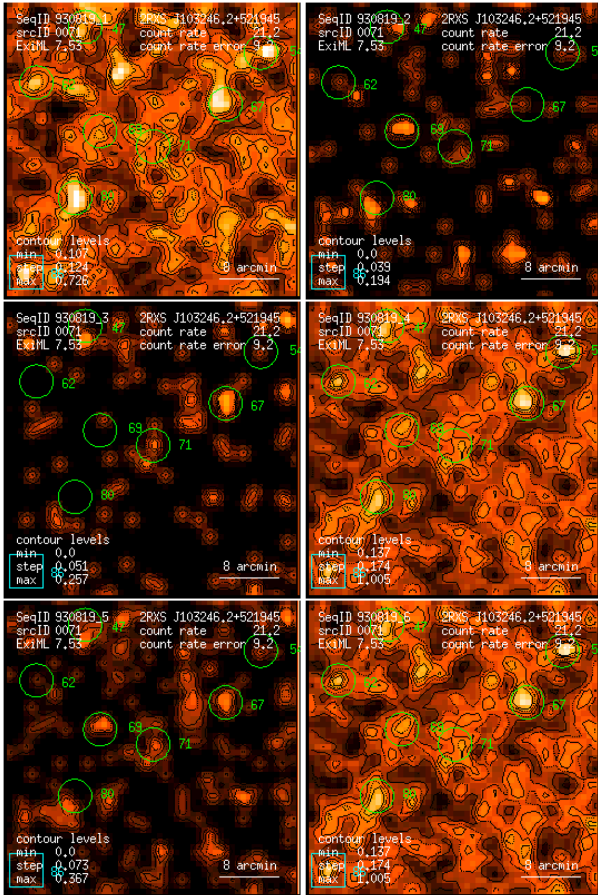
Figure 71: RASS 930819: detection 0071: band rate images, Gaussian filter: (1) PSPC channels 11 – 41, (2) 52 – 90, (3) 91 – 201, (4) 11 – 235, (5) 52 – 201, (6) 11 – 201. Broad band rates in counts/ks. Band rate contour levels in counts/ks/arcmin 2 .
