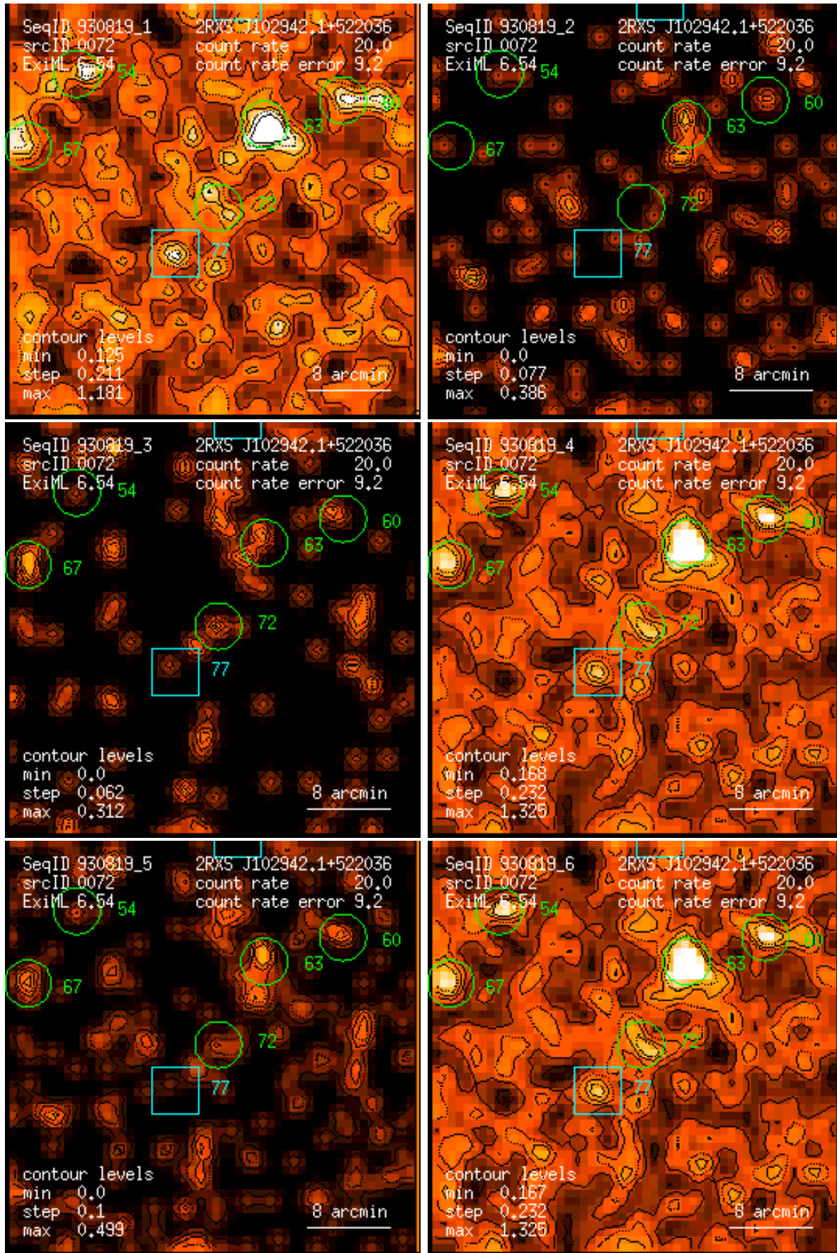
Figure 72: RASS 930819: detection 0072: band rate images, Gaussian filter: (1) PSPC channels 11 – 41, (2) 52 – 90, (3) 91 – 201, (4) 11 – 235, (5) 52 – 201, (6) 11 – 201. Broad band rates in counts/ks. Band rate contour levels in counts/ks/arcmin 2 .
