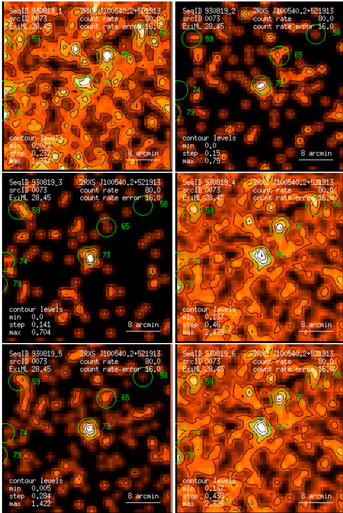
Figure 73: RASS 930819: detection 0073: band rate images, Gaussian filter: (1) PSPC channels 11 – 41, (2) 52 – 90, (3) 91 – 201, (4) 11 – 235, (5) 52 – 201, (6) 11 – 201. Broad band rates in counts/ks. Band rate contour levels in counts/ks/arcmin 2 .
