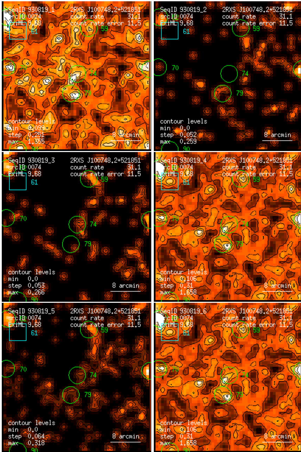
Figure 74: RASS 930819: detection 0074: band rate images, Gaussian filter: (1) PSPC channels 11 – 41, (2) 52 – 90, (3) 91 – 201, (4) 11 – 235, (5) 52 – 201, (6) 11 – 201. Broad band rates in counts/ks. Band rate contour levels in counts/ks/arcmin 2 .
