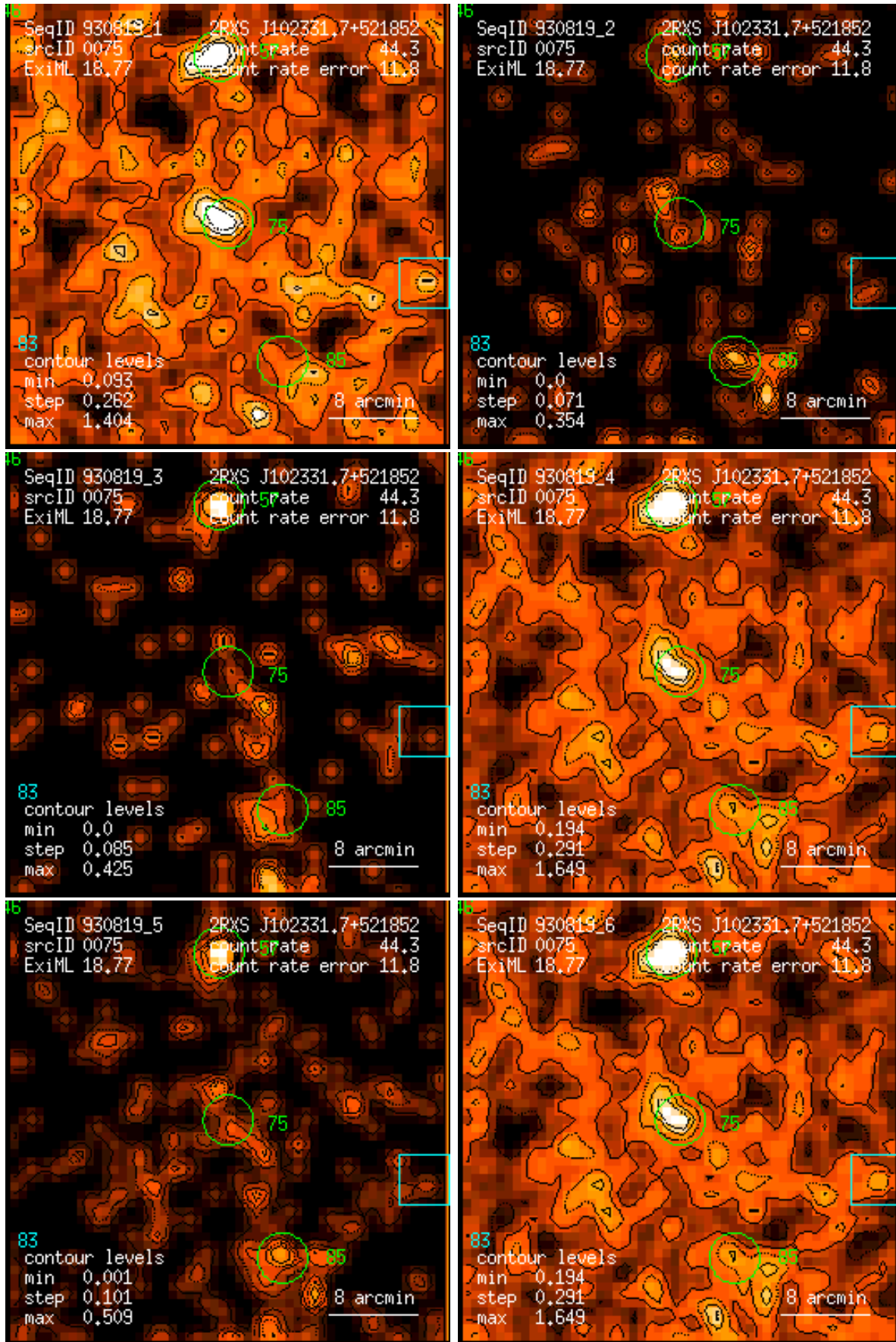
Figure 75: RASS 930819: detection 0075: band rate images, Gaussian filter: (1) PSPC channels 11 – 41, (2) 52 – 90, (3) 91 – 201, (4) 11 – 235, (5) 52 – 201, (6) 11 – 201. Broad band rates in counts/ks. Band rate contour levels in counts/ks/arcmin 2 .
