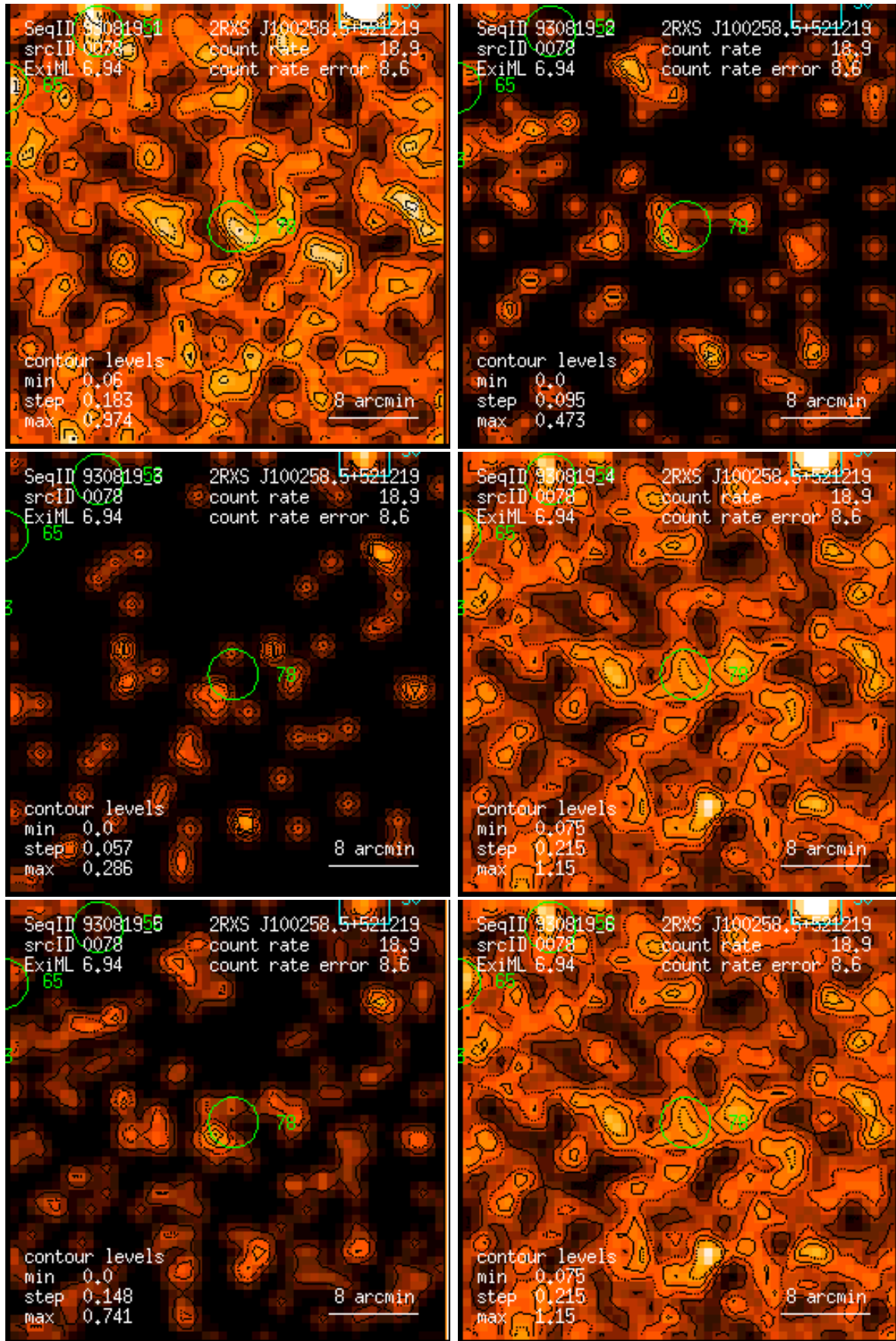
Figure 78: RASS 930819: detection 0078: band rate images, Gaussian filter: (1) PSPC channels 11 – 41, (2) 52 – 90, (3) 91 – 201, (4) 11 – 235, (5) 52 – 201, (6) 11 – 201. Broad band rates in counts/ks. Band rate contour levels in counts/ks/arcmin 2 .
