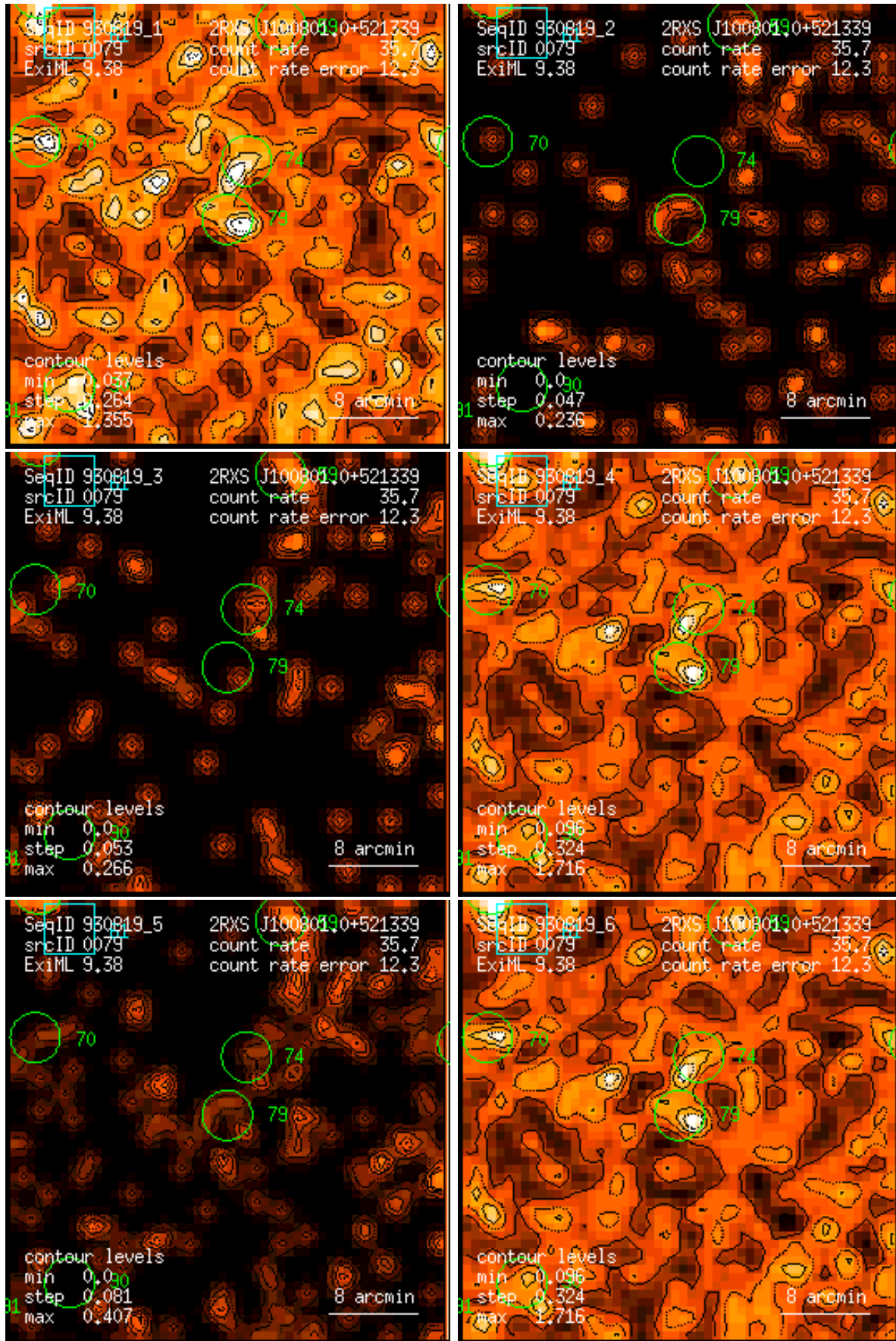
Figure 79: RASS 930819: detection 0079: band rate images, Gaussian filter: (1) PSPC channels 11 – 41, (2) 52 – 90, (3) 91 – 201, (4) 11 – 235, (5) 52 – 201, (6) 11 – 201. Broad band rates in counts/ks. Band rate contour levels in counts/ks/arcmin 2 .
