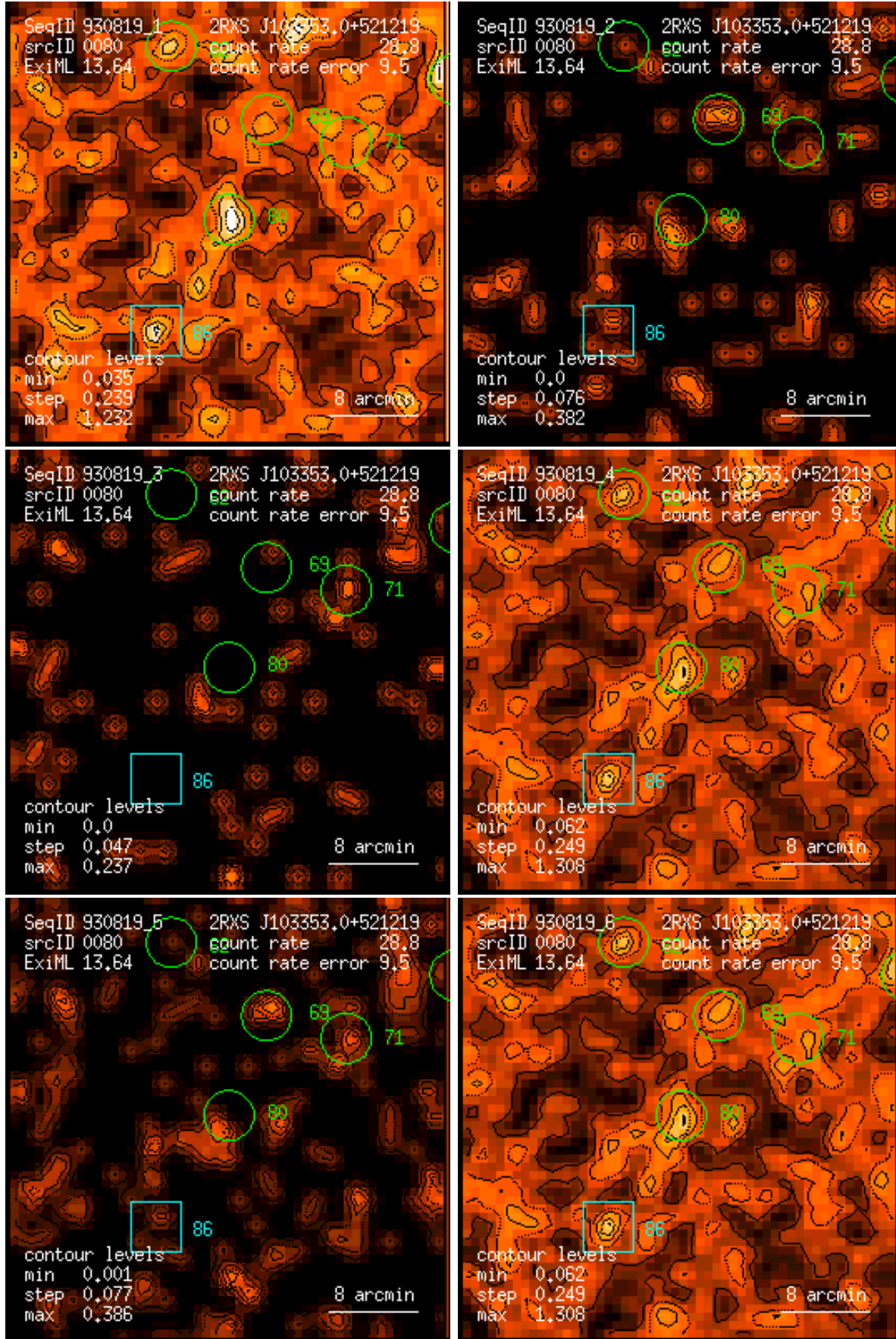
Figure 80: RASS 930819: detection 0080: band rate images, Gaussian filter: (1) PSPC channels 11 – 41, (2) 52 – 90, (3) 91 – 201, (4) 11 – 235, (5) 52 – 201, (6) 11 – 201. Broad band rates in counts/ks. Band rate contour levels in counts/ks/arcmin 2 .
