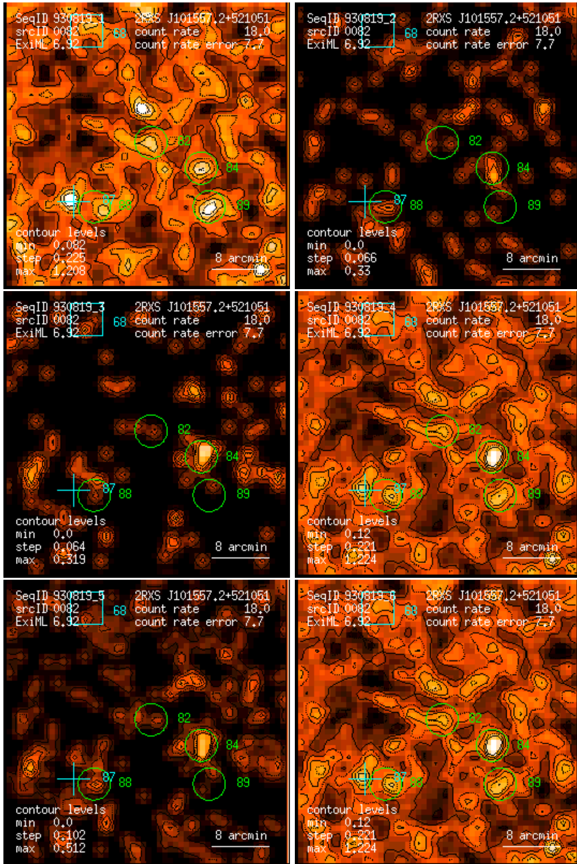
Figure 82: RASS 930819: detection 0082: band rate images, Gaussian filter: (1) PSPC channels 11 – 41, (2) 52 – 90, (3) 91 – 201, (4) 11 – 235, (5) 52 – 201, (6) 11 – 201. Broad band rates in counts/ks. Band rate contour levels in counts/ks/arcmin 2 .
