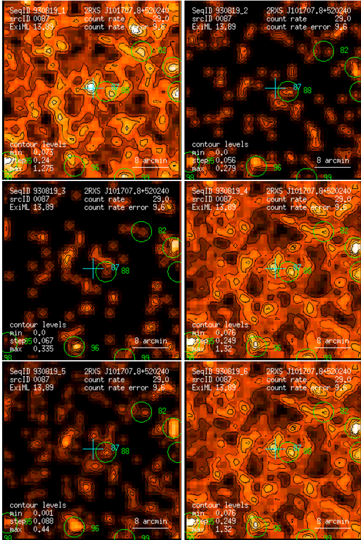
Figure 87: RASS 930819: detection 0087: band rate images, Gaussian filter: (1) PSPC channels 11 – 41, (2) 52 – 90, (3) 91 – 201, (4) 11 – 235, (5) 52 – 201, (6) 11 – 201. Broad band rates in counts/ks. Band rate contour levels in counts/ks/arcmin 2 .
