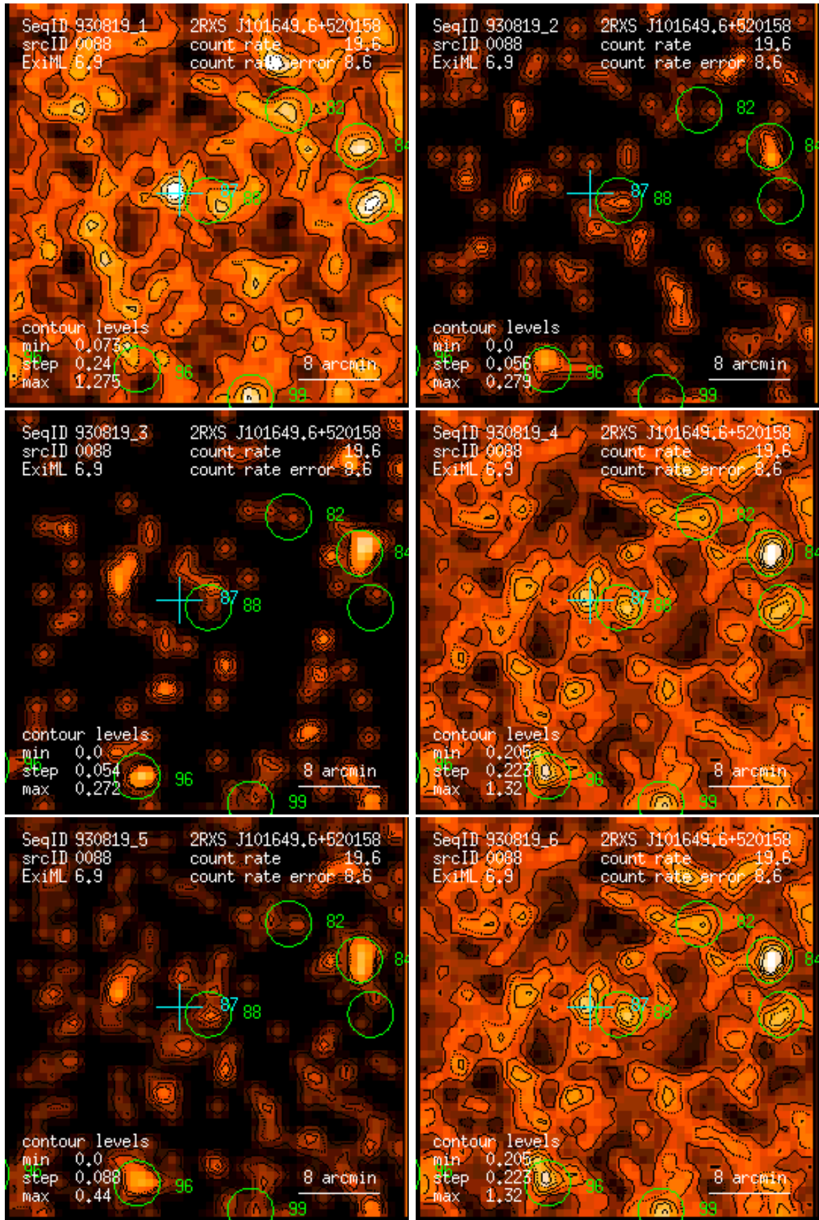
Figure 88: RASS 930819: detection 0088: band rate images, Gaussian filter: (1) PSPC channels 11 – 41, (2) 52 – 90, (3) 91 – 201, (4) 11 – 235, (5) 52 – 201, (6) 11 – 201. Broad band rates in counts/ks. Band rate contour levels in counts/ks/arcmin 2 .
