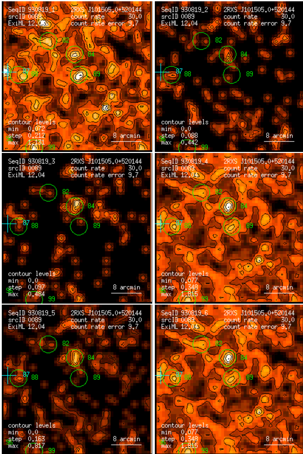
Figure 89: RASS 930819: detection 0089: band rate images, Gaussian filter: (1) PSPC channels 11 – 41, (2) 52 – 90, (3) 91 – 201, (4) 11 – 235, (5) 52 – 201, (6) 11 – 201. Broad band rates in counts/ks. Band rate contour levels in counts/ks/arcmin 2 .
