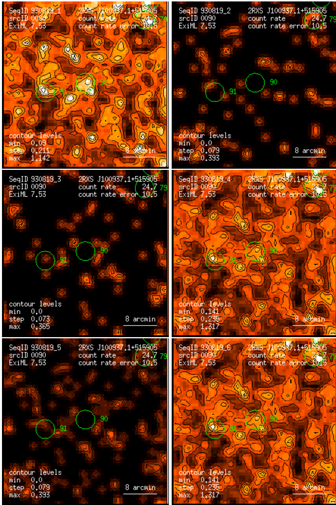
Figure 90: RASS 930819: detection 0090: band rate images, Gaussian filter: (1) PSPC channels 11 – 41, (2) 52 – 90, (3) 91 – 201, (4) 11 – 235, (5) 52 – 201, (6) 11 – 201. Broad band rates in counts/ks. Band rate contour levels in counts/ks/arcmin 2 .
