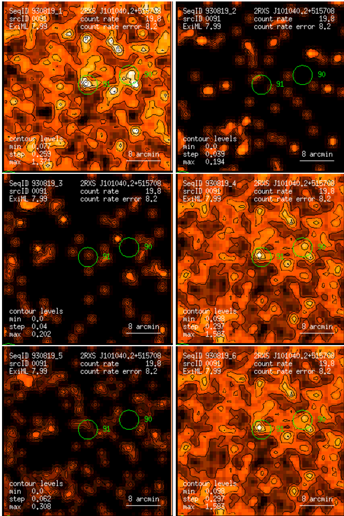
Figure 91: RASS 930819: detection 0091: band rate images, Gaussian filter: (1) PSPP channels 11 – 41, (2) 52 – 90, (3) 91 – 201, (4) 11 – 235, (5) 52 – 201, (6) 11 – 201. Broad band rates in counts/ks. Band rate contour levels in counts/ks/arcmin 2 .
