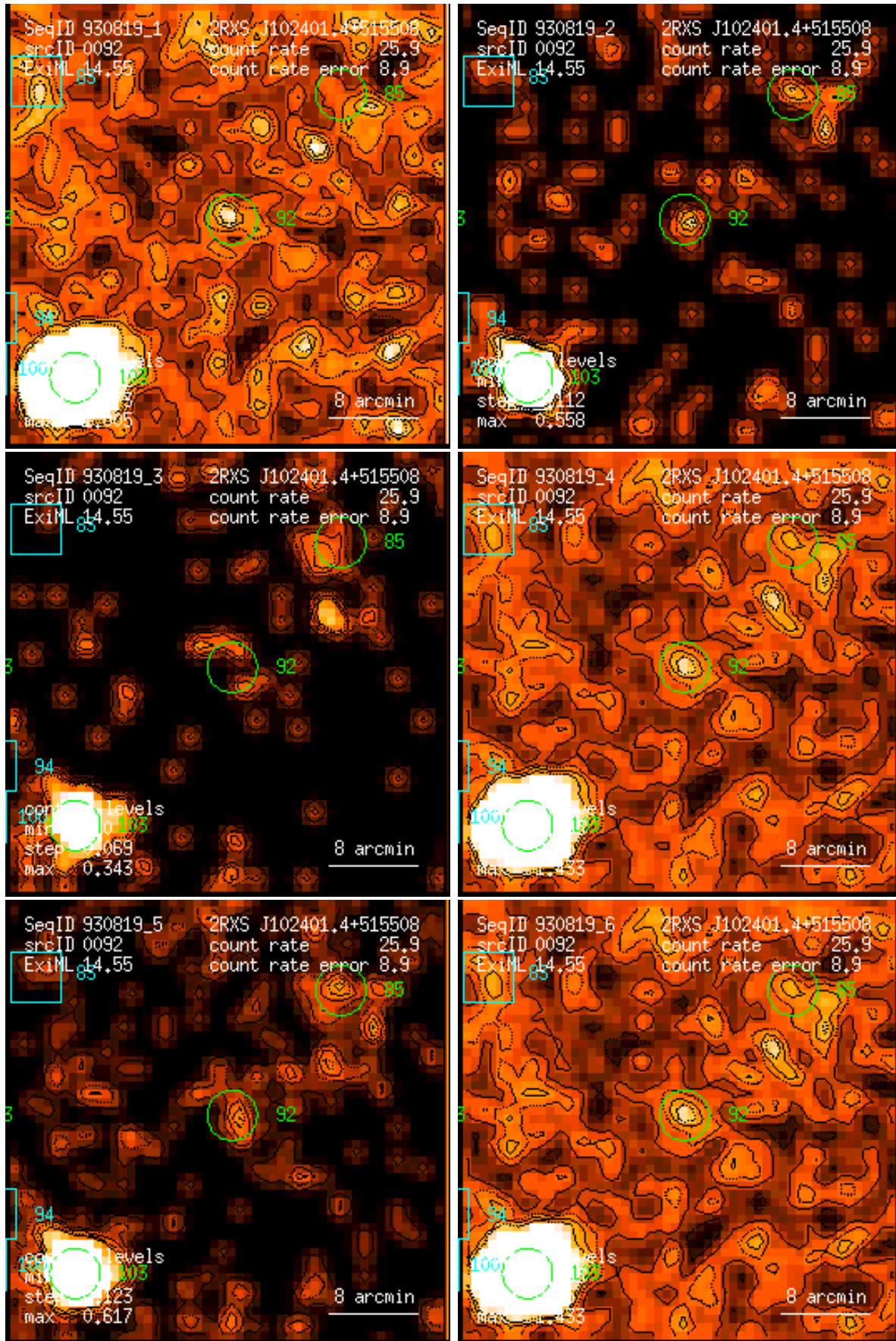
Figure 92: RASS 930819: detection 0092: band rate images, Gaussian filter: (1) PSPC channels 11 – 41, (2) 52 – 90, (3) 91 – 201, (4) 11 – 235, (5) 52 – 201, (6) 11 – 201. Broad band rates in counts/ks. Band rate contour levels in counts/ks/arcmin 2 .
