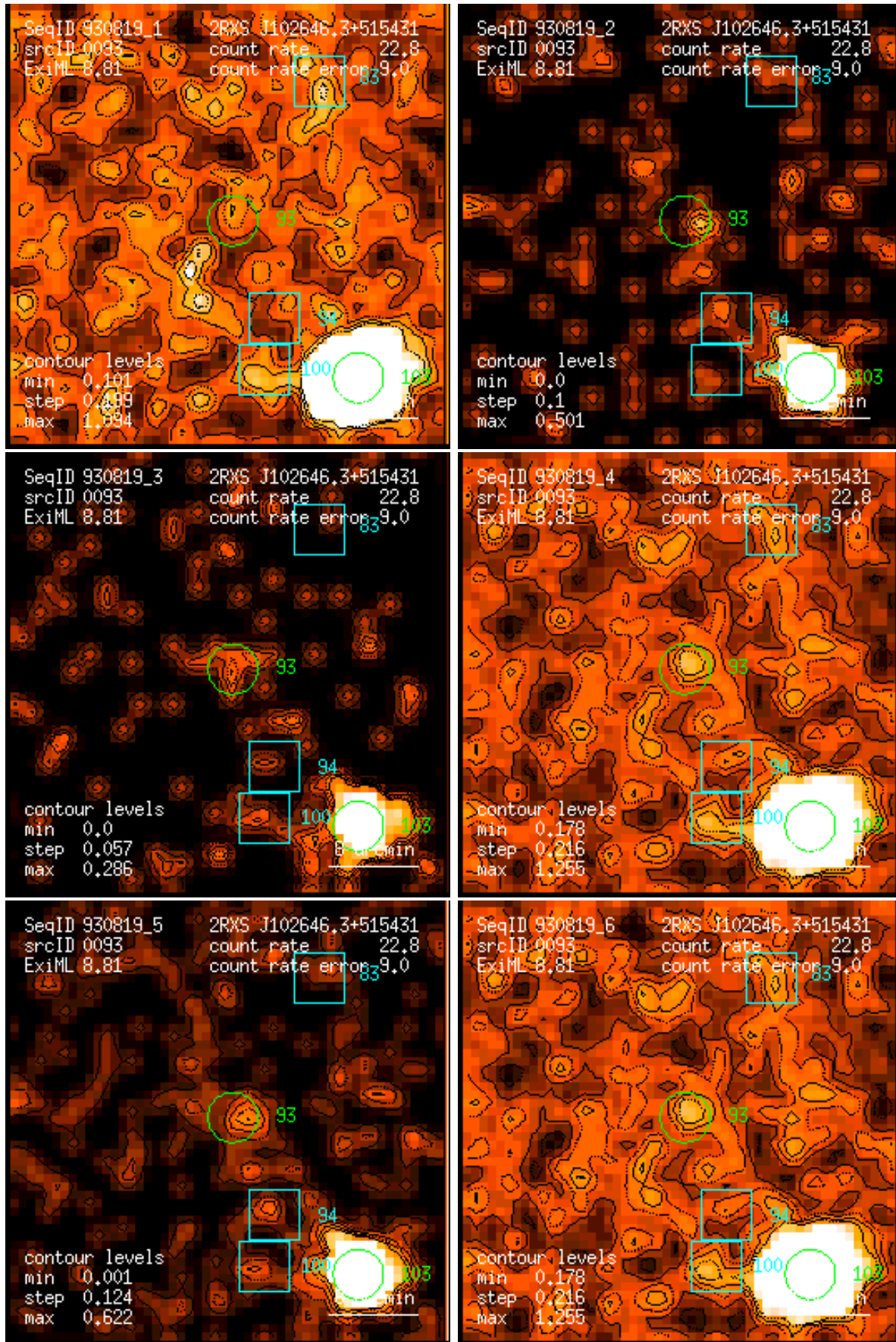
Figure 93: RASS 930819: detection 0093: band rate images, Gaussian filter: (1) PSPC channels 11 – 41, (2) 52 – 90, (3) 91 – 201, (4) 11 – 235, (5) 52 – 201, (6) 11 – 201. Broad band rates in counts/ks. Band rate contour levels in counts/ks/arcmin 2 .
