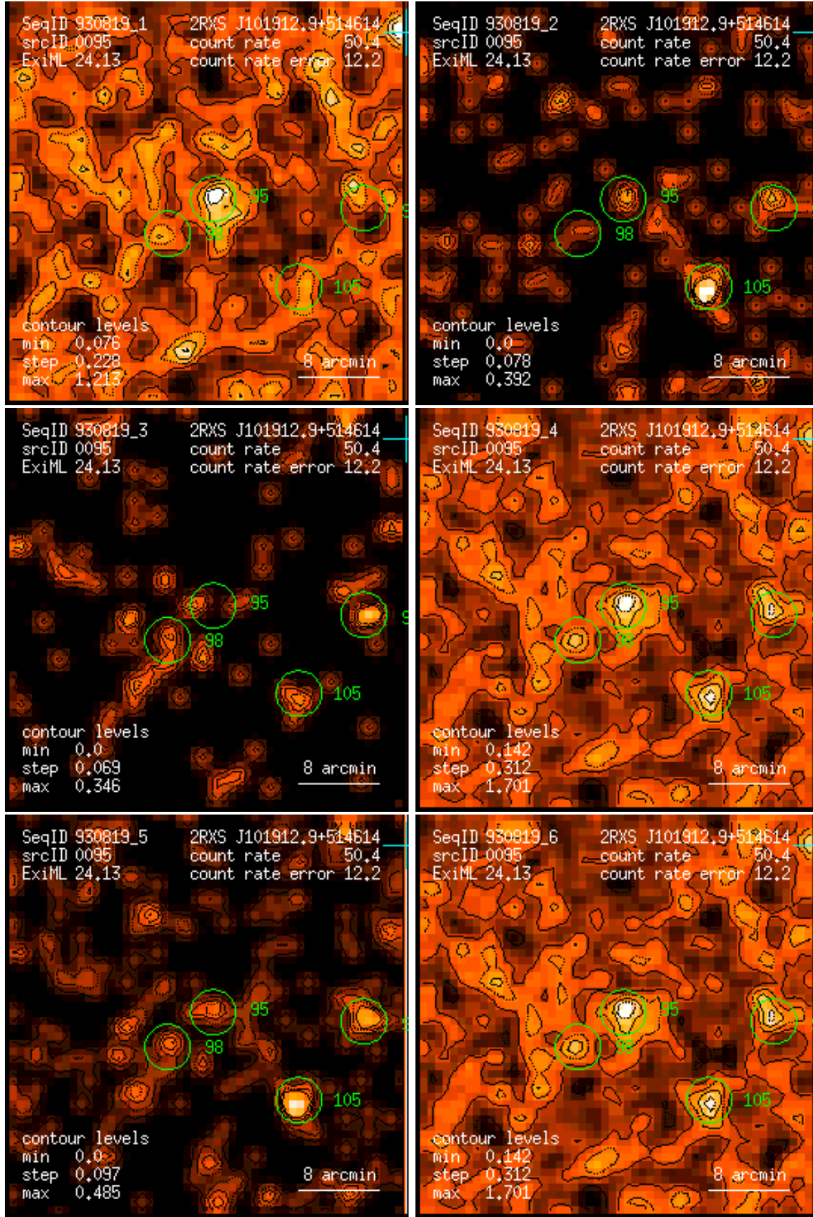
Figure 95: RASS 930819: detection 0095: band rate images, Gaussian filter: (1) PSPC channels 11 – 41, (2) 52 – 90, (3) 91 – 201, (4) 11 – 235, (5) 52 – 201, (6) 11 – 201. Broad band rates in counts/ks. Band rate contour levels in counts/ks/arcmin 2 .
