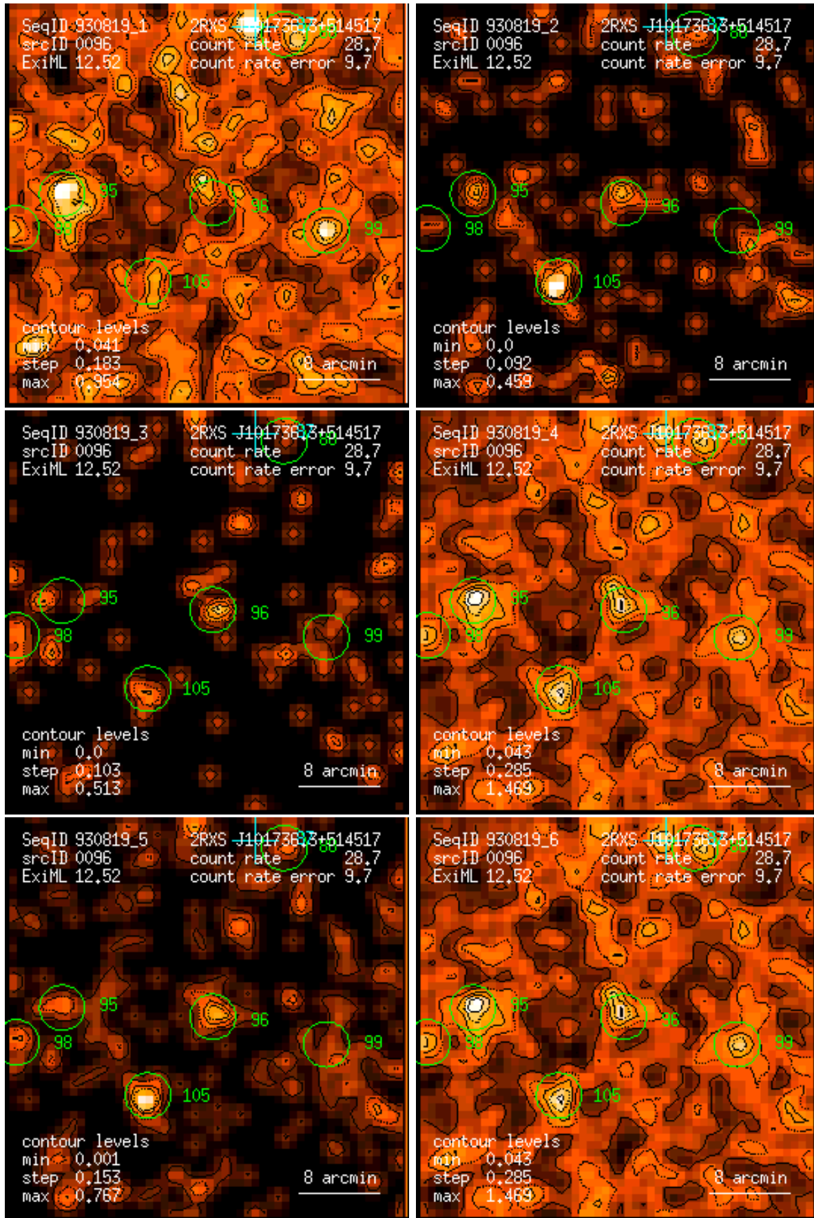
Figure 96: RASS 930819: detection 0096: band rate images, Gaussian filter: (1) PSPC channels 11 – 41, (2) 52 – 90, (3) 91 – 201, (4) 11 – 235, (5) 52 – 201, (6) 11 – 201. Broad band rates in counts/ks. Band rate contour levels in counts/ks/arcmin 2 .
