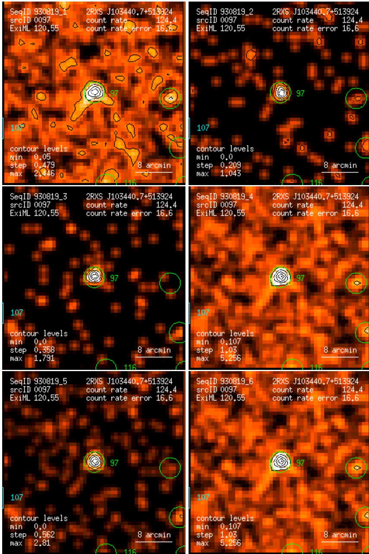
Figure 97: RASS 930819: detection 0097: band rate images, Gaussian filter: (1) PSPC channels 11 – 41, (2) 52 – 90, (3) 91 – 201, (4) 11 – 235, (5) 52 – 201, (6) 11 – 201. Broad band rates in counts/ks. Band rate contour levels in counts/ks/arcmin 2 .
