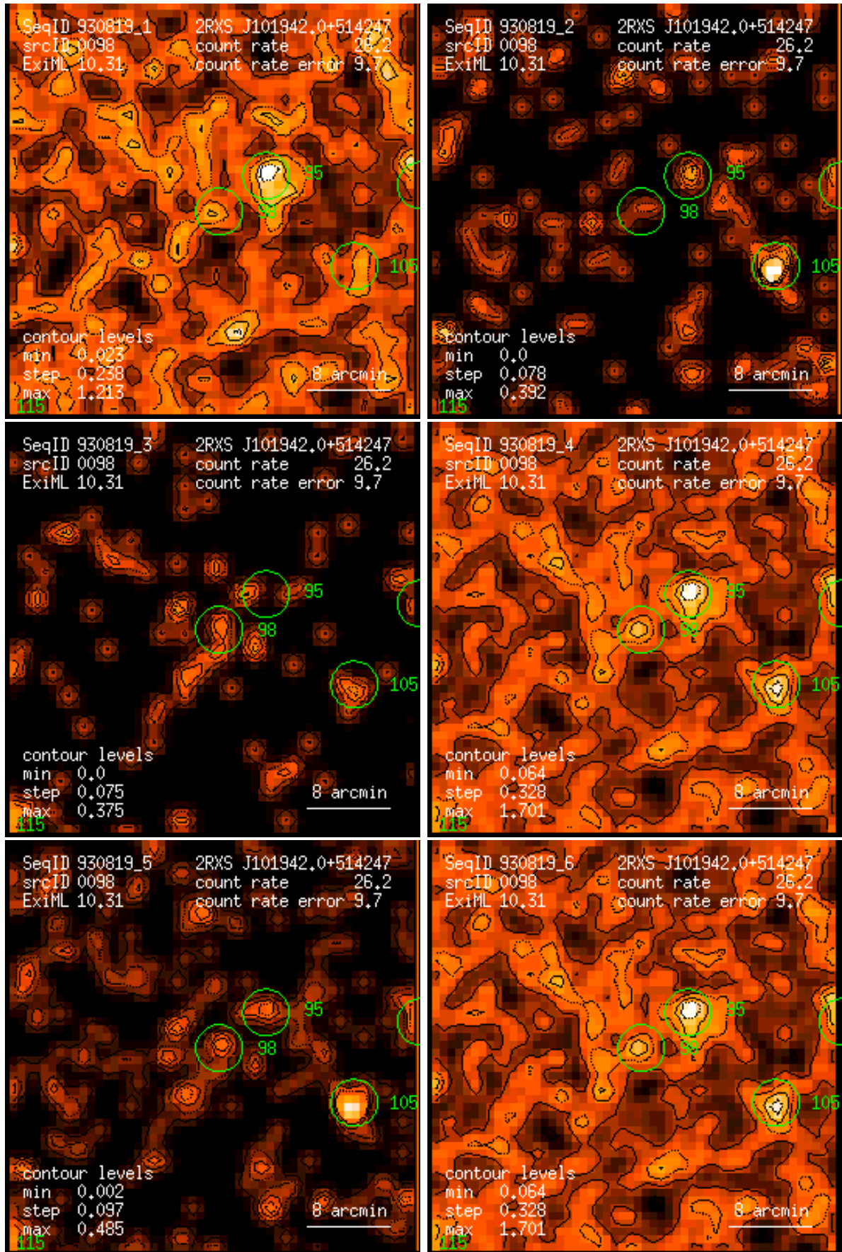
Figure 98: RASS 930819: detection 0098: band rate images, Gaussian filter: (1) PSPC channels 11 – 41, (2) 52 – 90, (3) 91 – 201, (4) 11 – 235, (5) 52 – 201, (6) 11 – 201. Broad band rates in counts/ks. Band rate contour levels in counts/ks/arcmin 2 .
