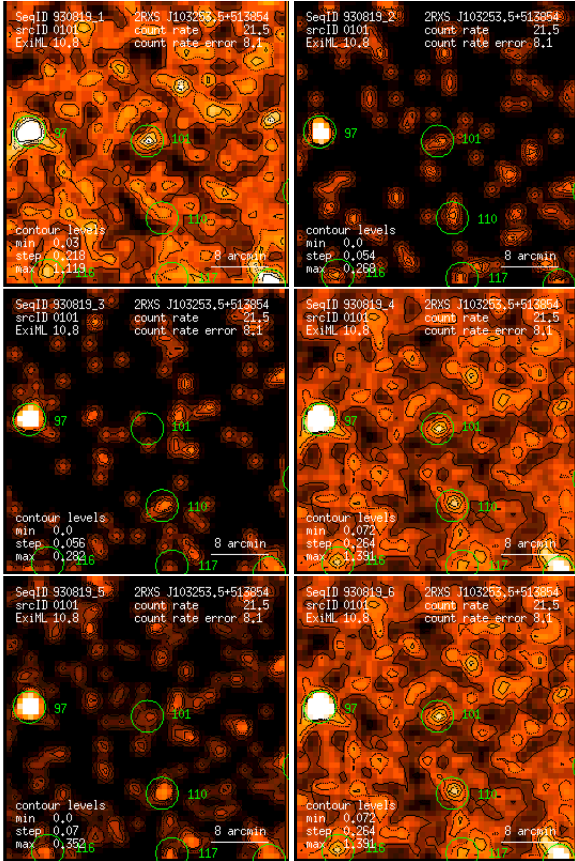
Figure 101: RASS 930819: detection 0101: band rate images, Gaussian filter: (1) PSPC channels 11 – 41, (2) 52 – 90, (3) 91 – 201, (4) 11 – 235, (5) 52 – 201, (6) 11 – 201. Broad band rates in counts/ks. Band rate contour levels in counts/ks/arcmin 2 .
