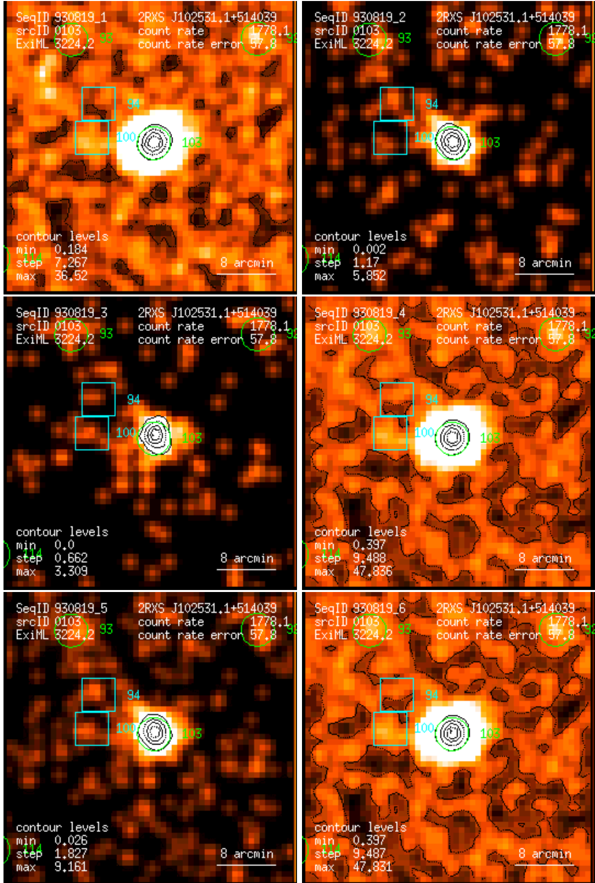
Figure 103: RASS 930819: detection 0103: band rate images, Gaussian filter: (1) PSPC channels 11 – 41, (2) 52 – 90, (3) 91 – 201, (4) 11 – 235, (5) 52 – 201, (6) 11 – 201. Broad band rates in counts/ks. Band rate contour levels in counts/ks/arcmin 2 .
