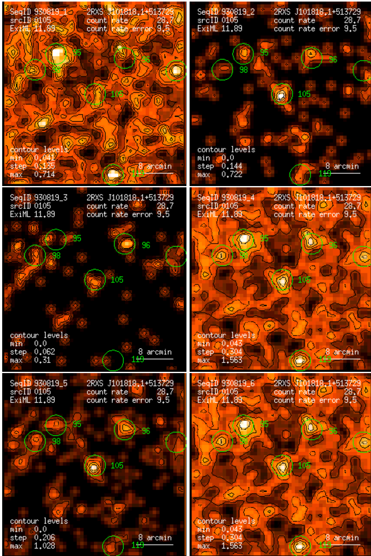
Figure 105: RASS 930819: detection 0105: band rate images, Gaussian filter: (1) PSPC channels 11 – 41, (2) 52 – 90, (3) 91 – 201, (4) 11 – 235, (5) 52 – 201, (6) 11 – 201. Broad band rates in counts/ks. Band rate contour levels in counts/ks/arcmin 2 .
