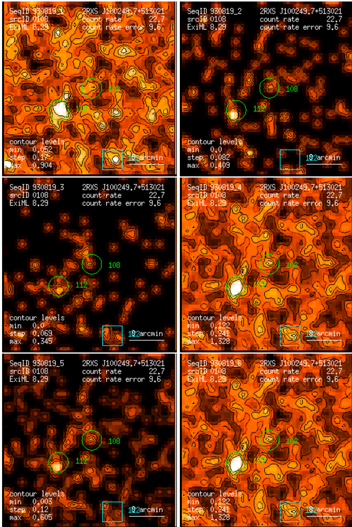
Figure 108: RASS 930819: detection 0108: band rate images, Gaussian filter: (1) PSPC channels 11 – 41, (2) 52 – 90, (3) 91 – 201, (4) 11 – 235, (5) 52 – 201, (6) 11 – 201. Broad band rates in counts/ks. Band rate contour levels in counts/ks/arcmin 2 .
