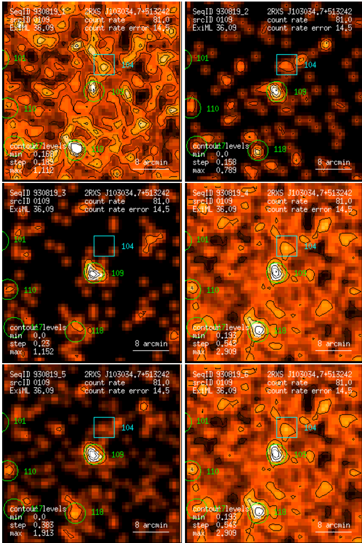
Figure 109: RASS 930819: detection 0109: band rate images, Gaussian filter: (1) PSPC channels 11 – 41, (2) 52 – 90, (3) 91 – 201, (4) 11 – 235, (5) 52 – 201, (6) 11 – 201. Broad band rates in counts/ks. Band rate contour levels in counts/ks/arcmin 2 .
