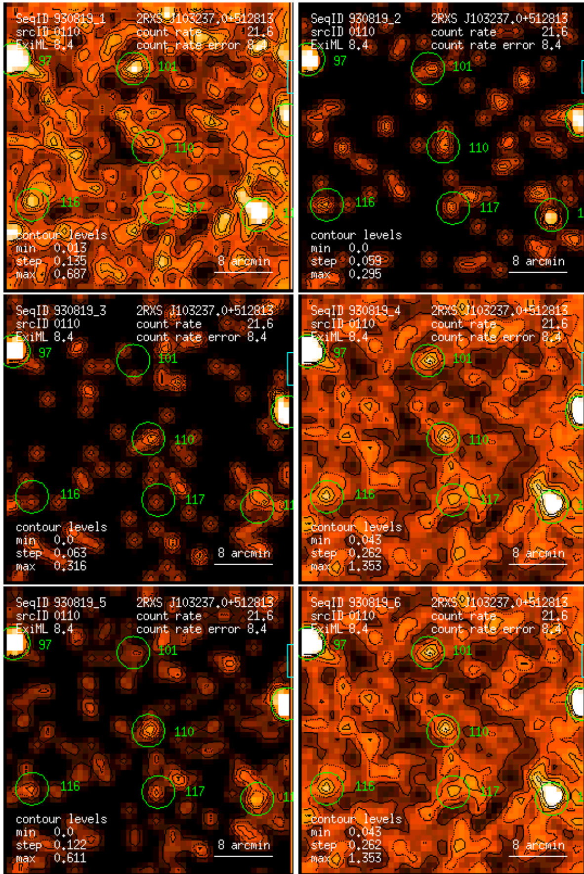
Figure 110: RASS 930819: detection 0110: band rate images, Gaussian filter: (1) PSPC channels 11 – 41, (2) 52 – 90, (3) 91 – 201, (4) 11 – 235, (5) 52 – 201, (6) 11 – 201. Broad band rates in counts/ks. Band rate contour levels in counts/ks/arcmin 2 .
