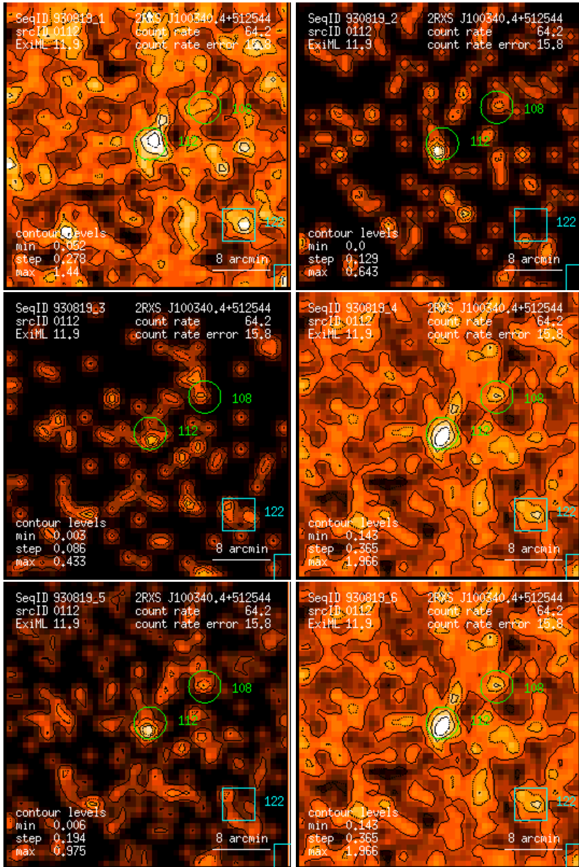
Figure 112: RASS 930819: detection 0112: band rate images, Gaussian filter: (1) PSPC channels 11 – 41, (2) 52 – 90, (3) 91 – 201, (4) 11 – 235, (5) 52 – 201, (6) 11 – 201. Broad band rates in counts/ks. Band rate contour levels in counts/ks/arcmin 2 .
